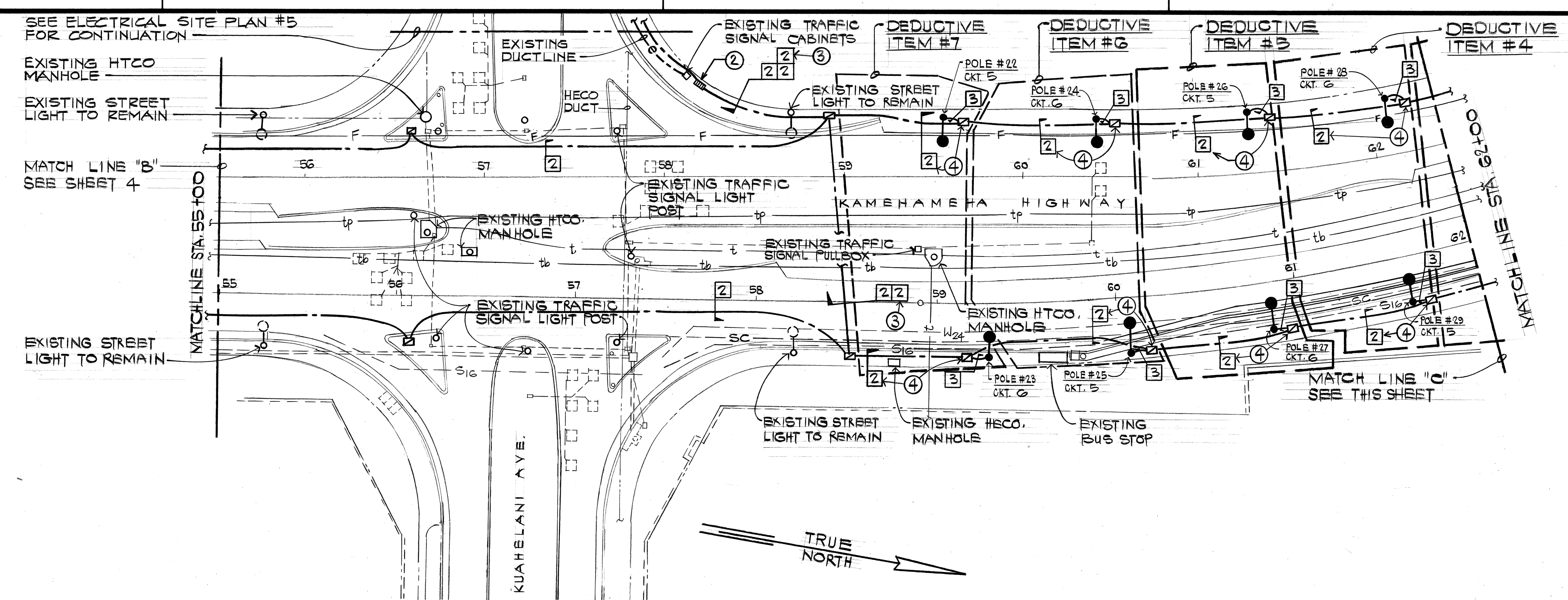
ELECTRICAL SITE PLAN #3 SCALE: 1" = 40'-0"
