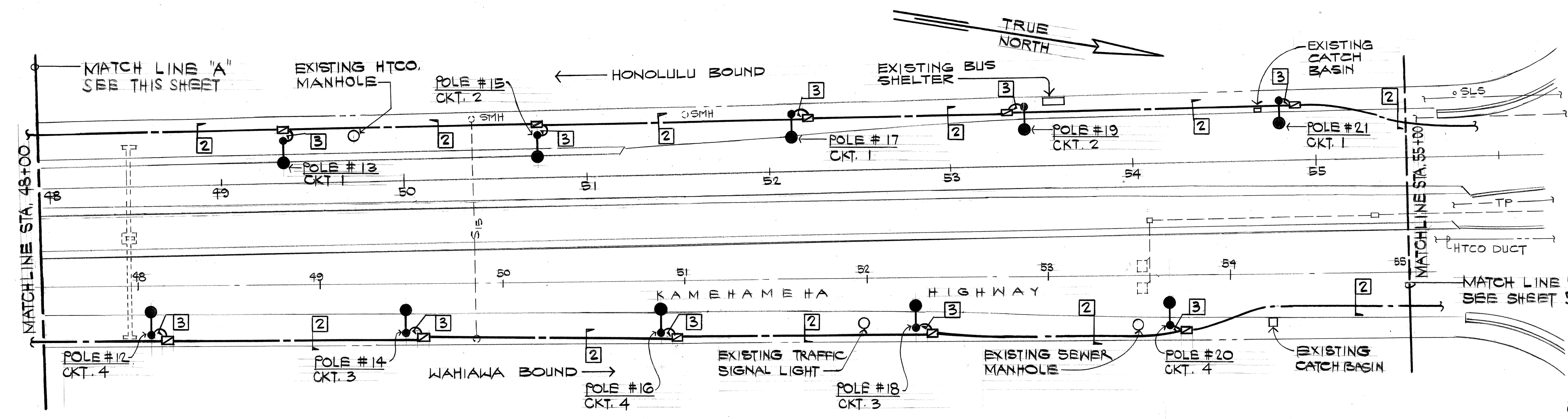
ELECTRICAL SITE PLAN #2 SCALE: 1" = 40'-0"
