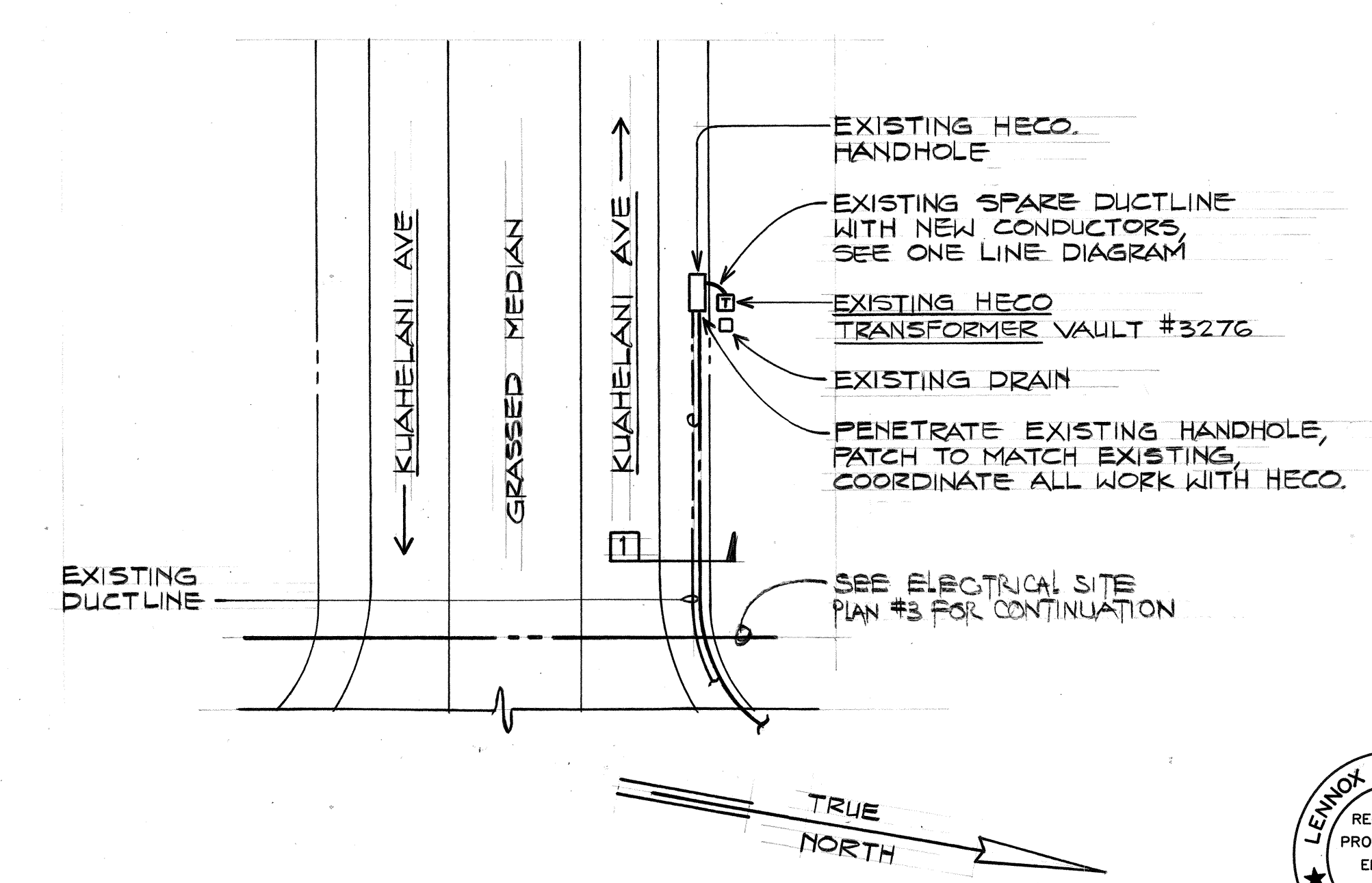
ELECTRICAL SITE PLAN #5 SCALE: 1" = 40'-0"
