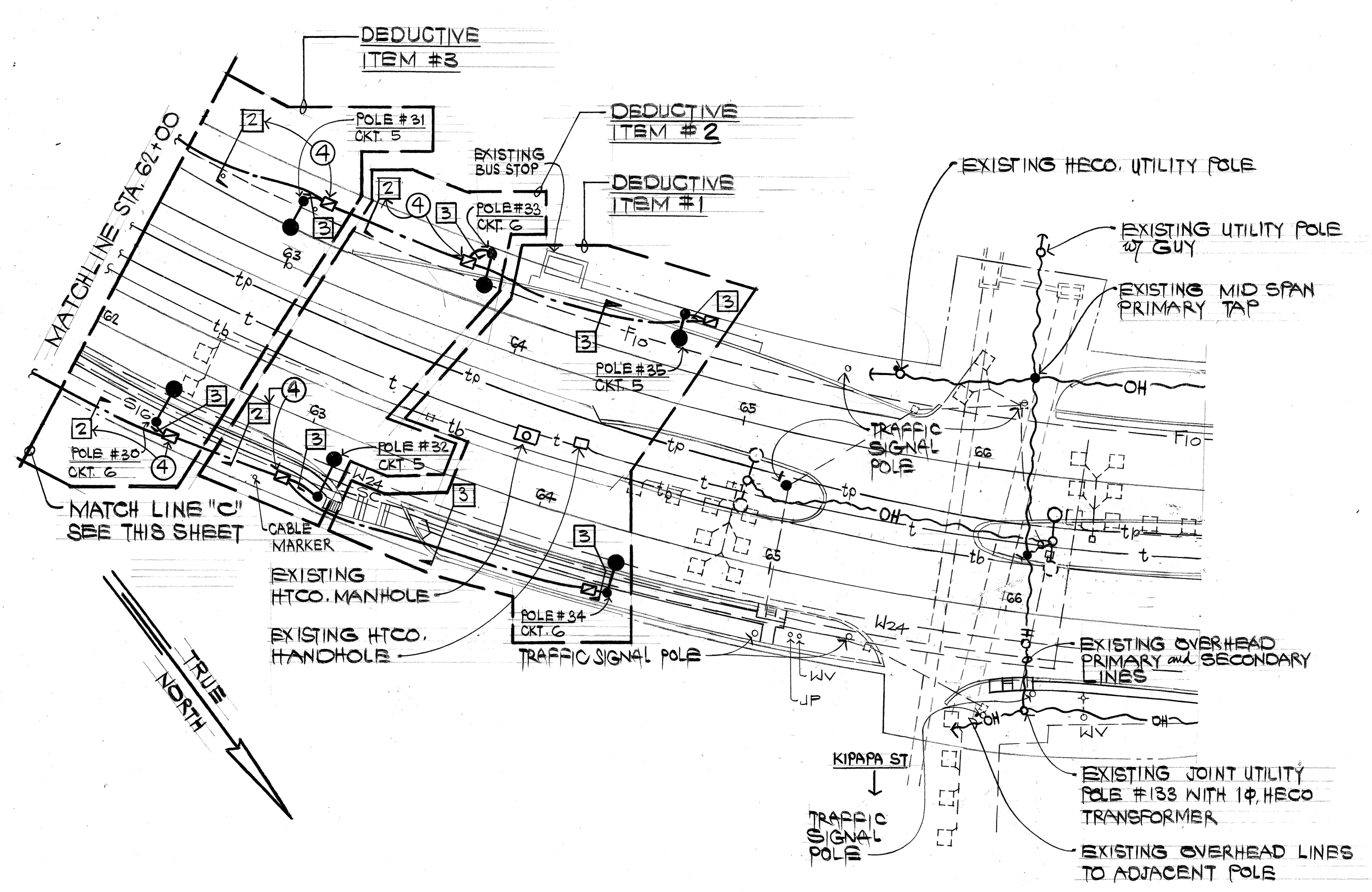
ELECTRICAL SITE PLAN #4 SCALE: 1" = 40'-0"
