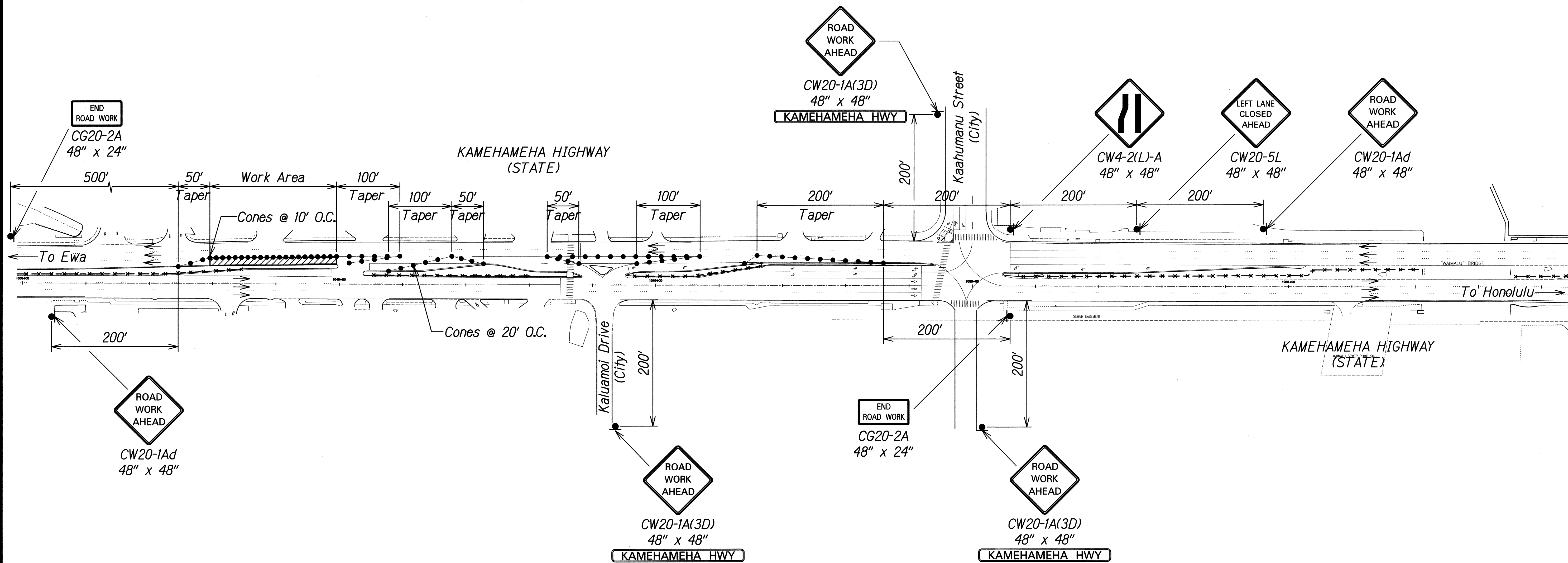
TYPICAL TRAFFIC CONTROL PLAN FOR WORK ZONE IN EWA BOUND LANES Not to Scale
