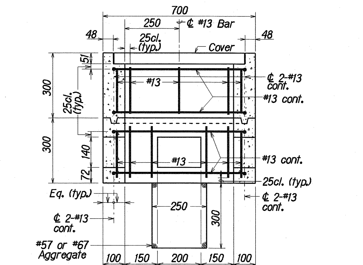
TYPE "B" PULLBOX (Old Type "C") Scale: 1 : 100
