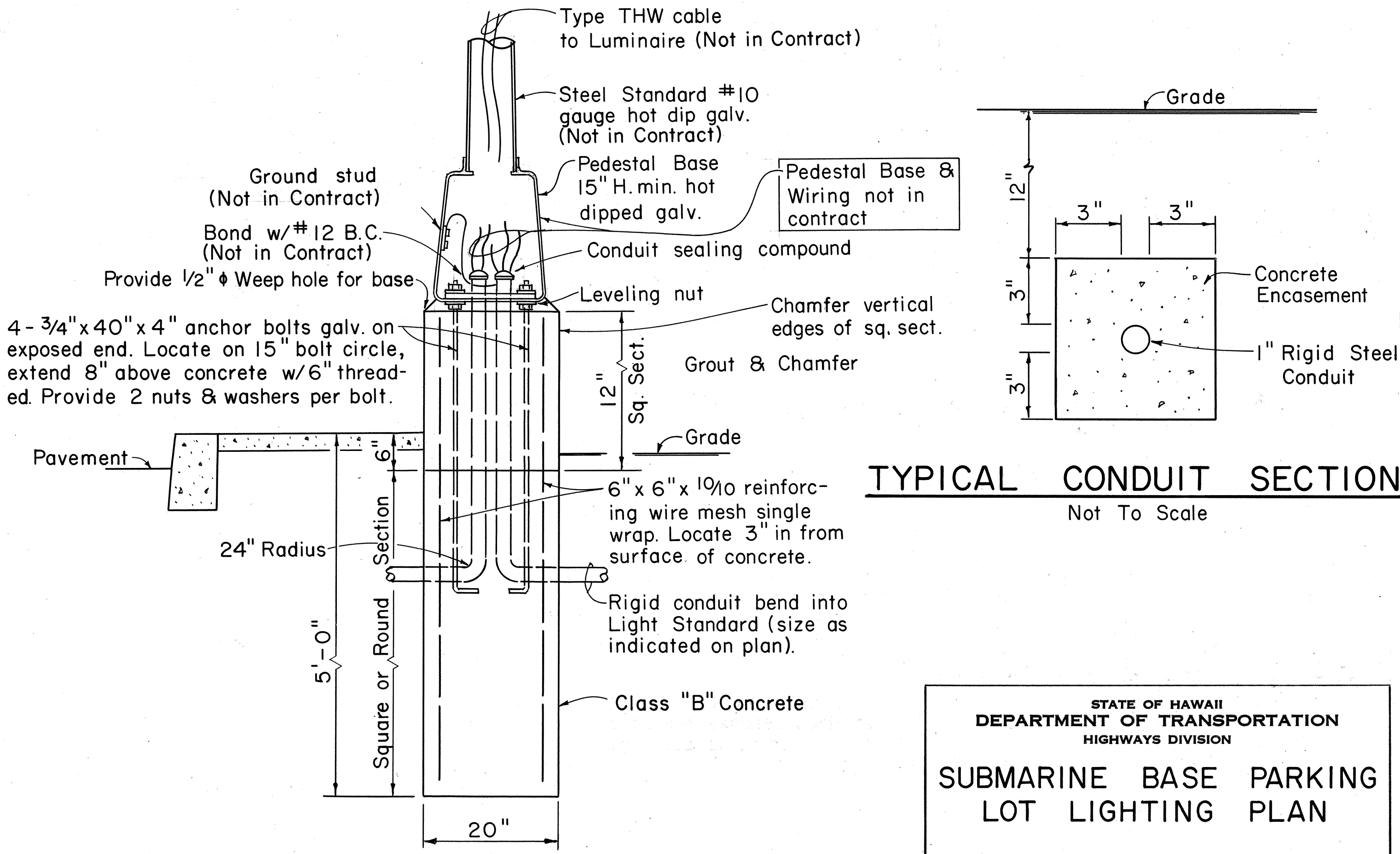
POLE AND FOUNDATION DETAIL Not To Scale
