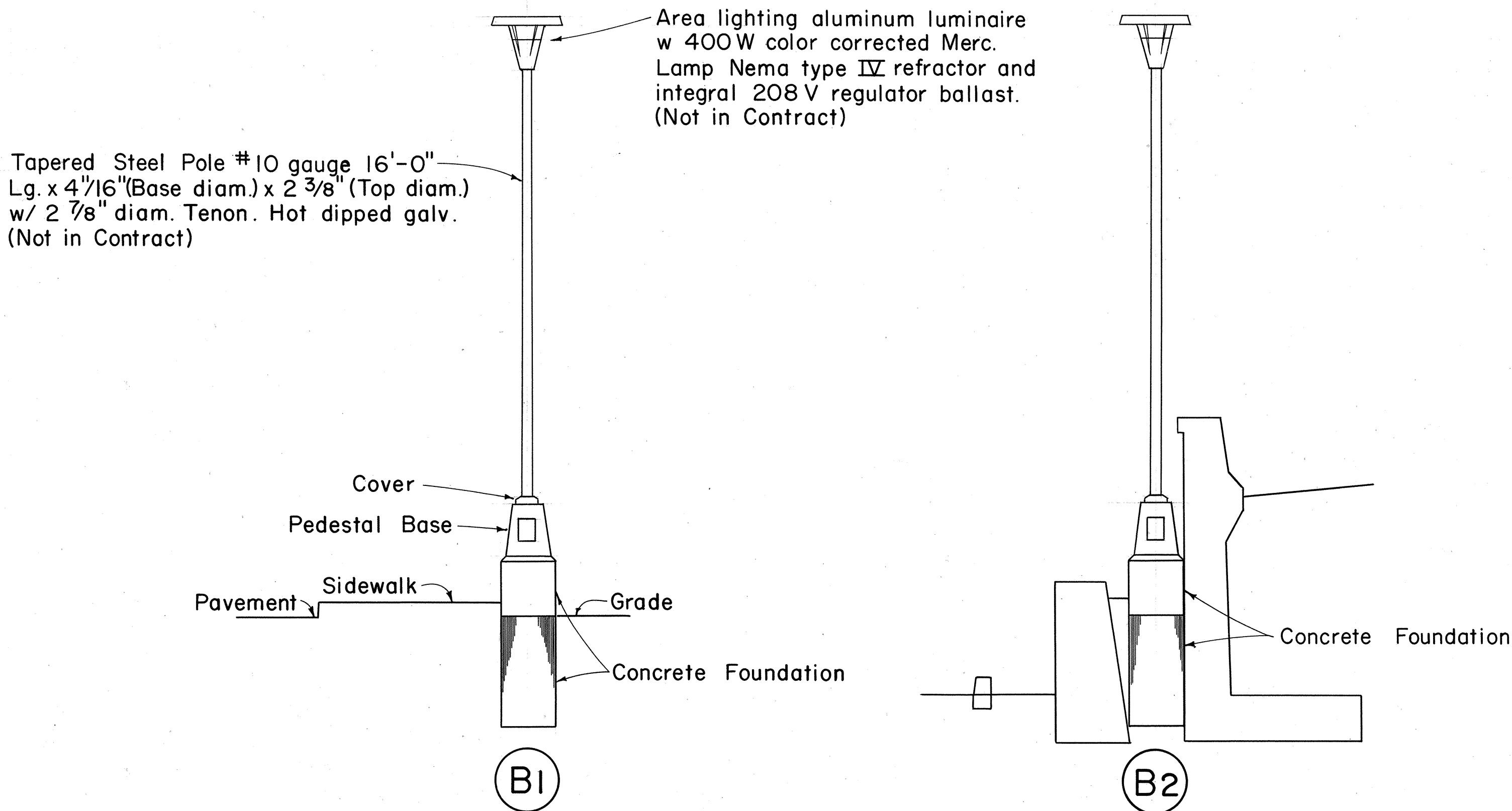
LIGHTING STANDARD ELEVATIONS Not To Scale
