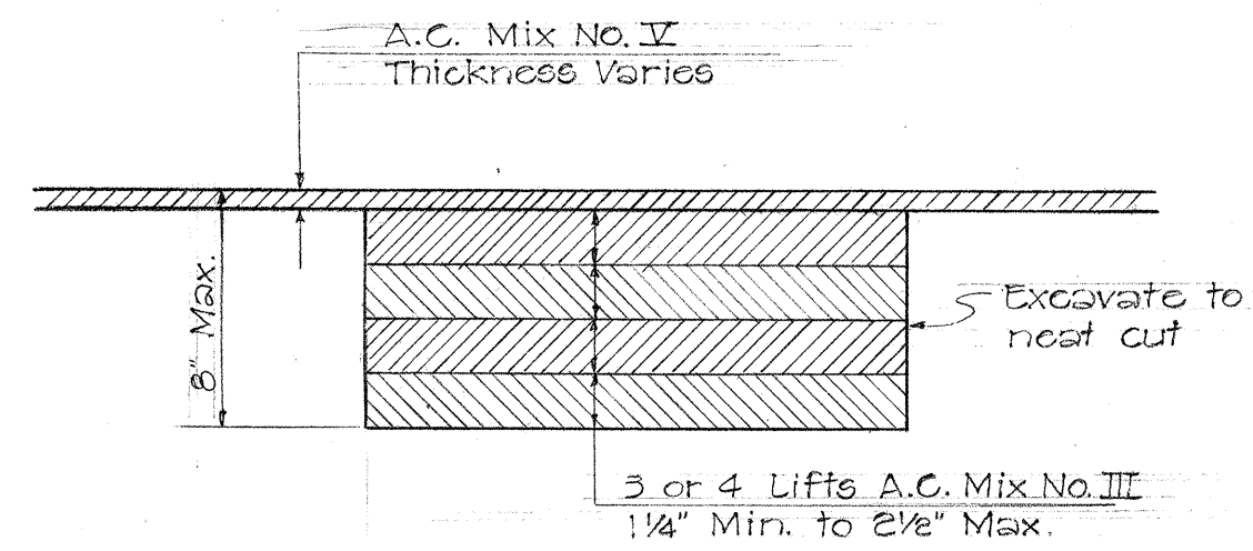
TYPICAL SECTION OF RECONSTRUCTION Not to Scale
