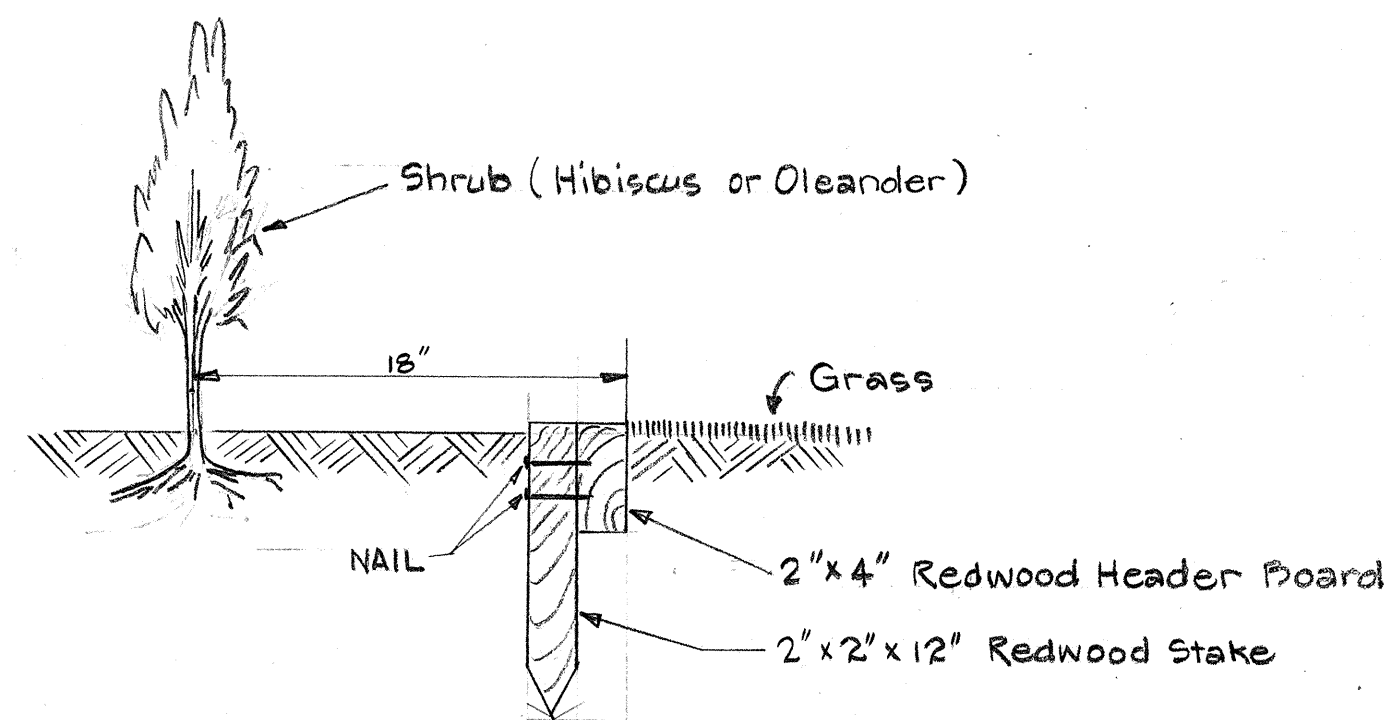
TYPICAL DETAIL REDWOOD HEADER BOARD
