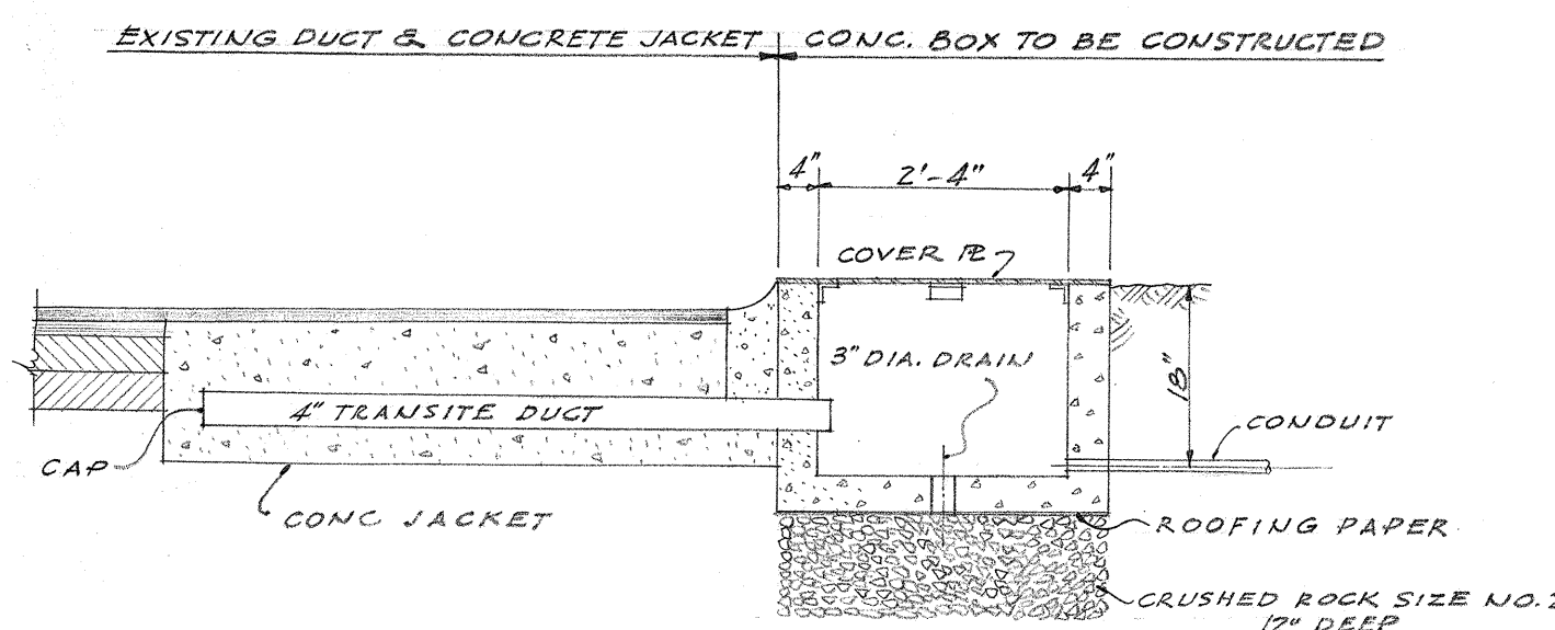
TRAFFIC DETECTOR JUNCTION BOX AND DUCT SCALE: 1/2" = 1'-0"
