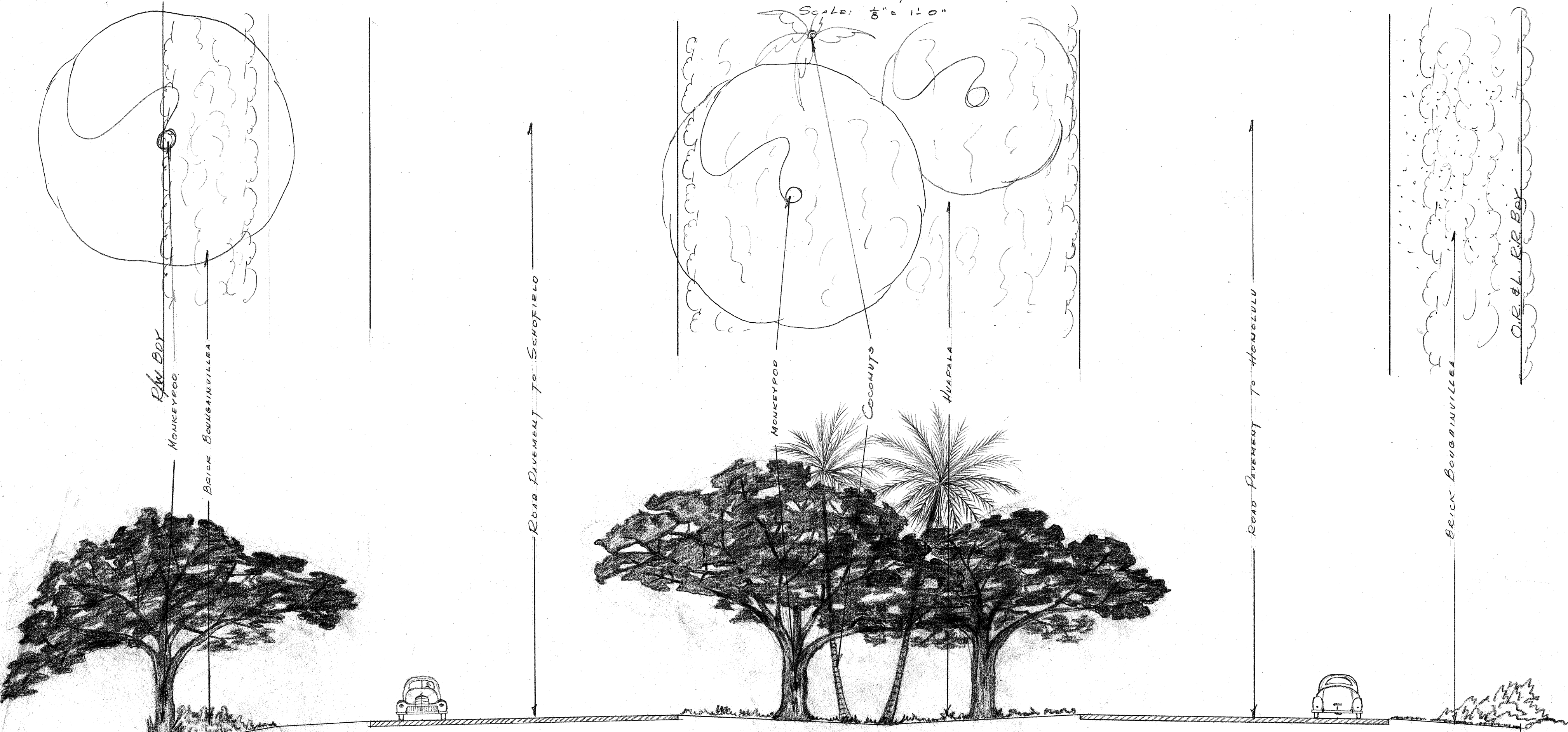
TYPICAL CROSS SECTION OF ROADSIDE PLANTING AT APPROACHES TO INTERSECTIONS Scale: 1" = 50' 0"
