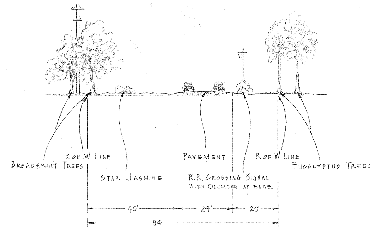
CROSS SECTION OF TYPICAL PLANTING AT STATION 23
