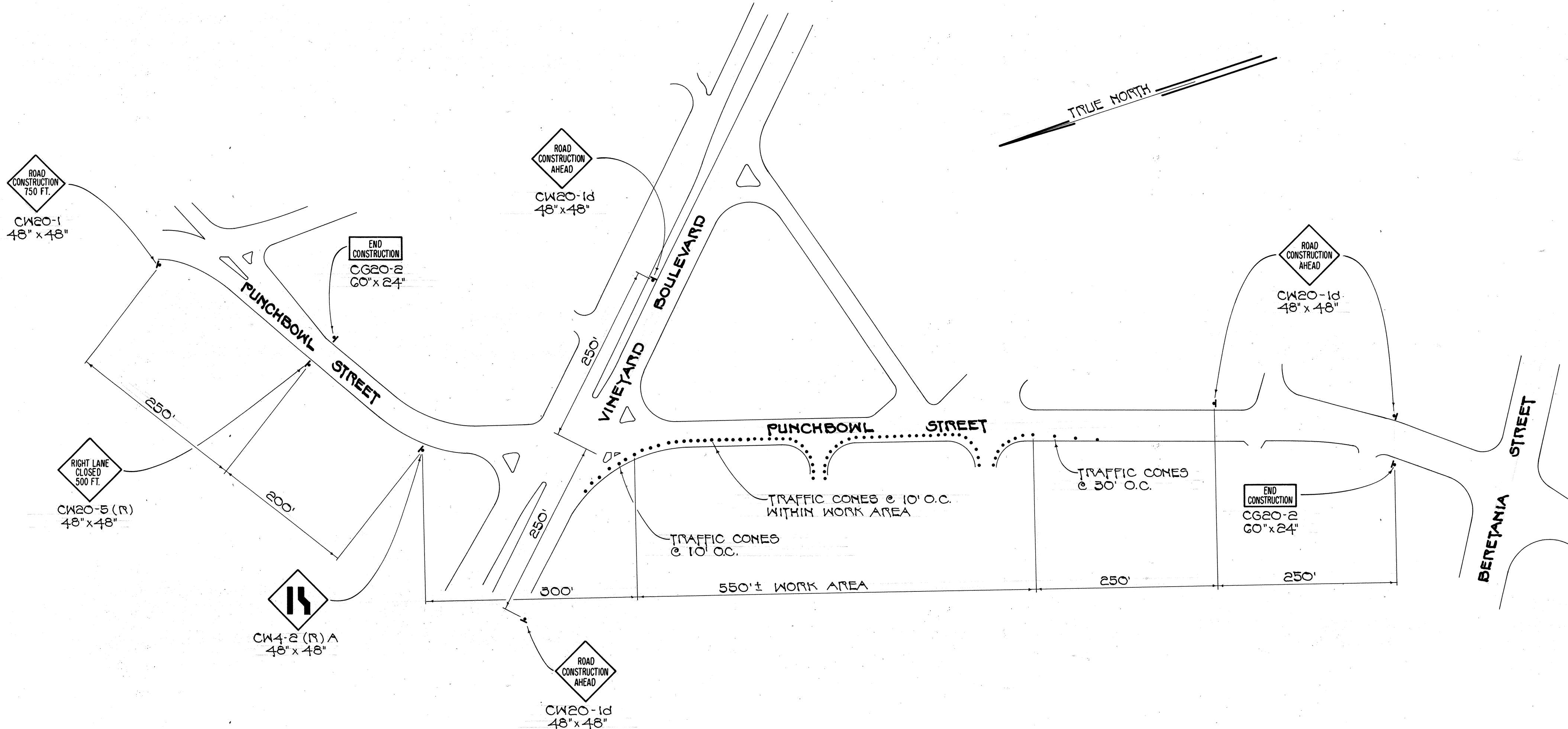
TRAFFIC CONTROL PLAN NOT TO SCALE
