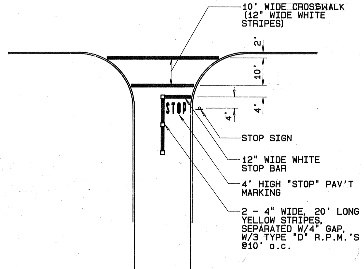
TYPICAL STRIPING/SIGNING DETAIL AT INTERSECTIONS WITHIN CITY & COUNTY R/W ONLY
