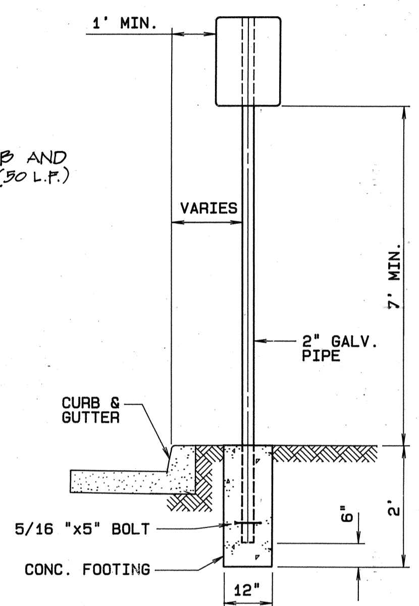
TYPICAL SIGN POST DETAIL WITHIN CITY & COUNTY R/W ONLY
