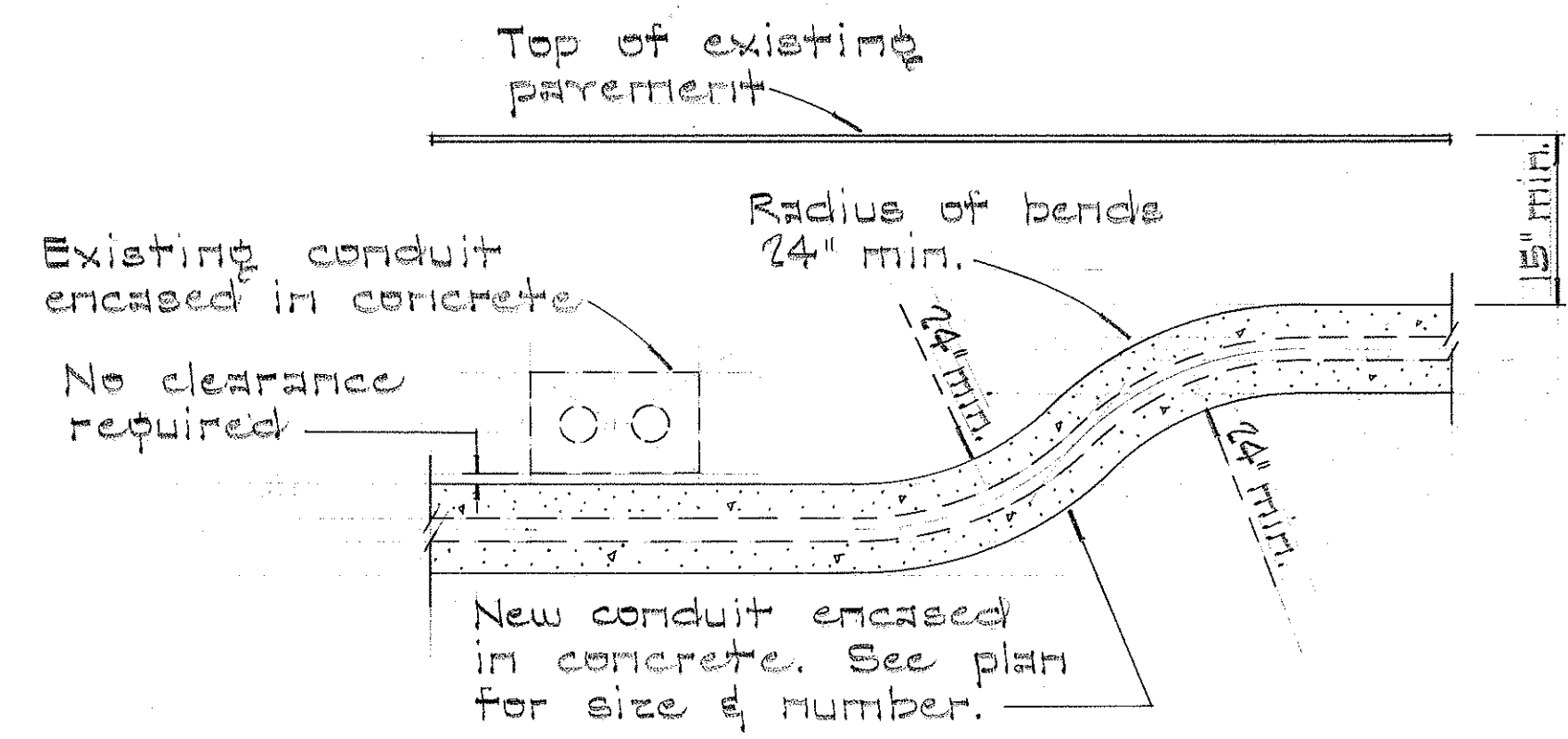
TYPICAL DETAIL OF EXISTING CONDUIT BY-PASS Not to Scale
