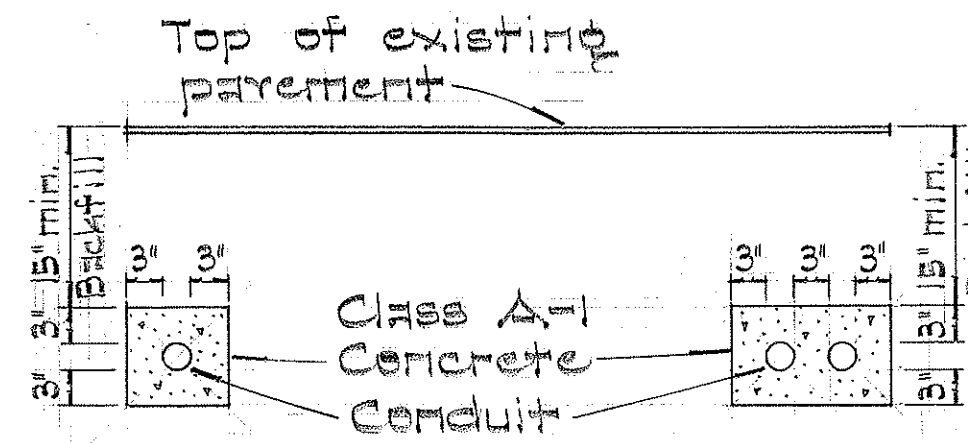
TYPICAL DETAIL OF CONDUITS ENCASED IN CONCRETE Not to Scale
