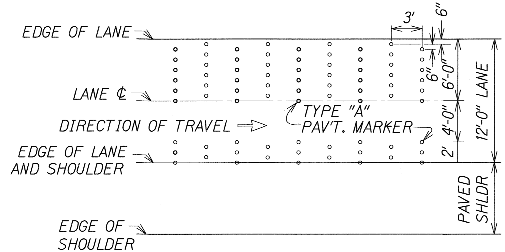
TYPICAL RUMBLE STRIP DETAIL Scale: 1"=4'-0"
