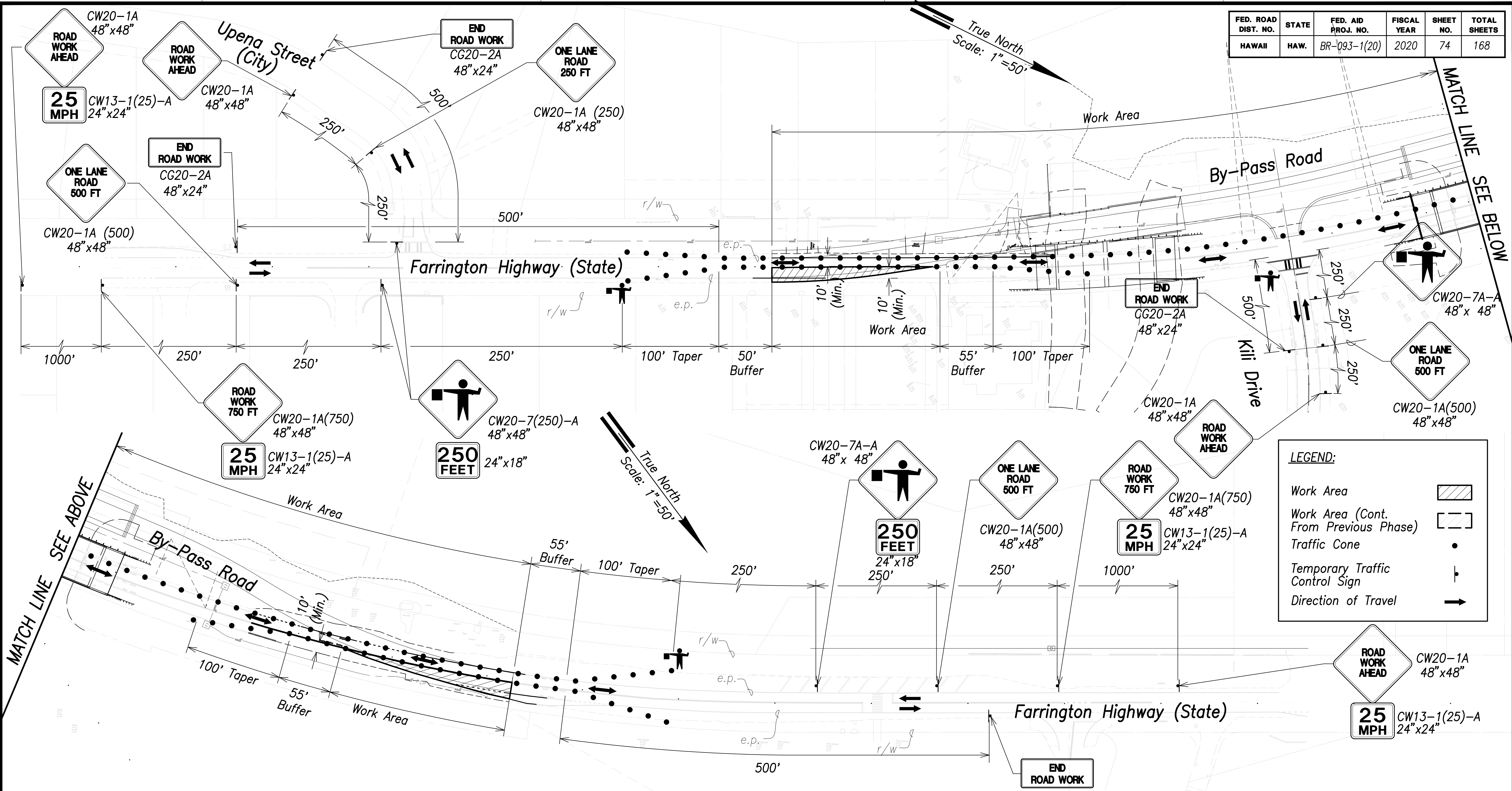
TRAFFIC CONTROL PLAN - 3 Scale: 1"=50'
