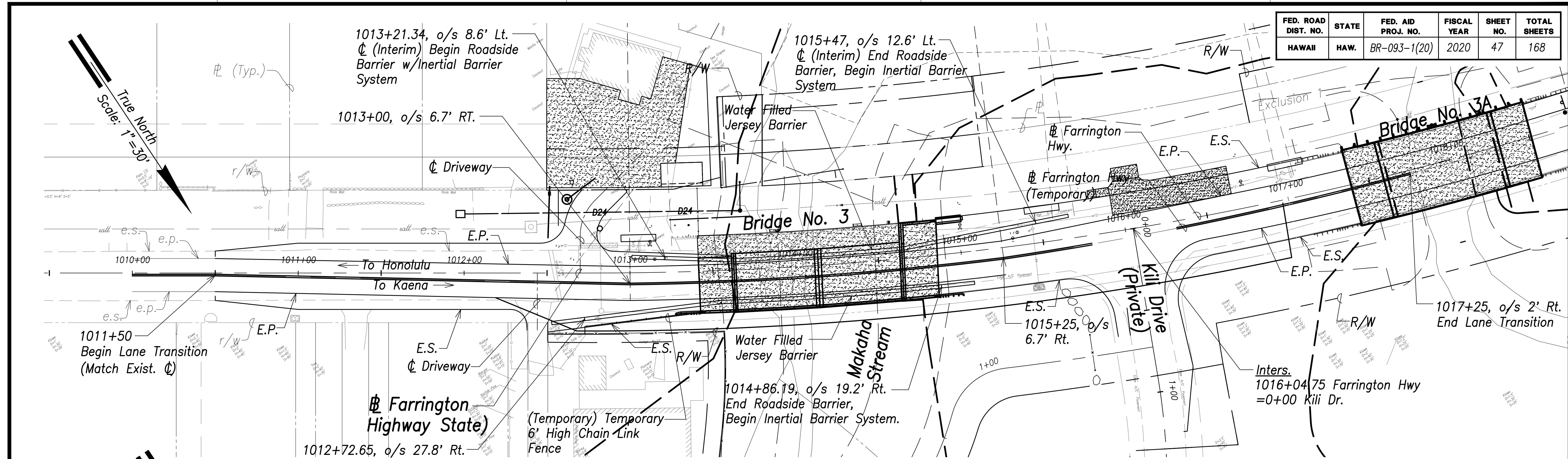
INTERIM SITE AND GEOMETRIC PLAN Scale: 1"=30'
