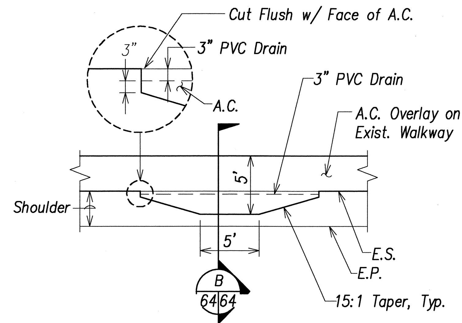
PASSING SPACE AT A.C. WALKWAY (SHOULDER SIDE) SCALE: 1" = 5' 4 Various 64
