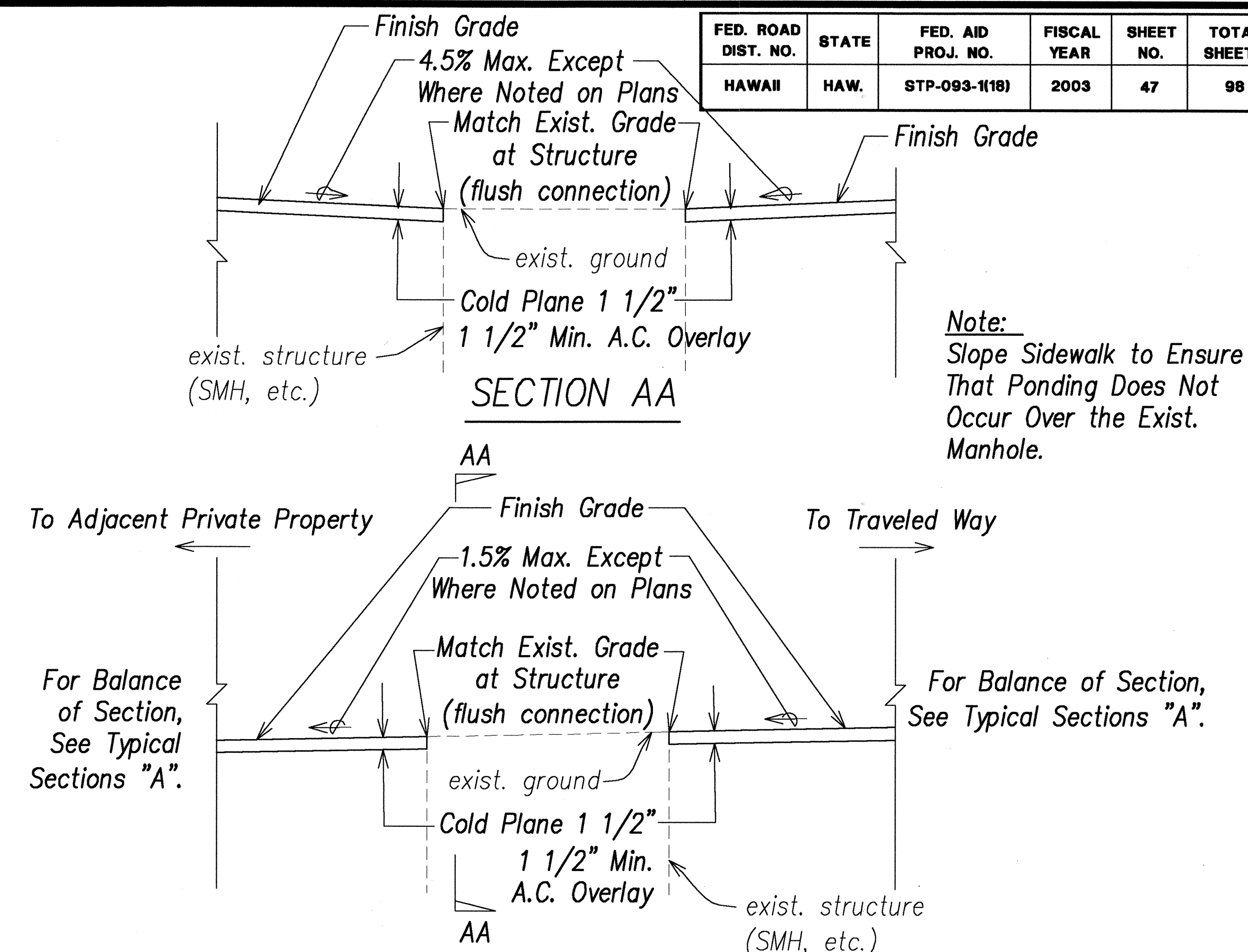
Various 47 TYPICAL SECTIONS - TRANSITION AT EXISTING STRUCTURE SCALE: 1" = 1'-0"
