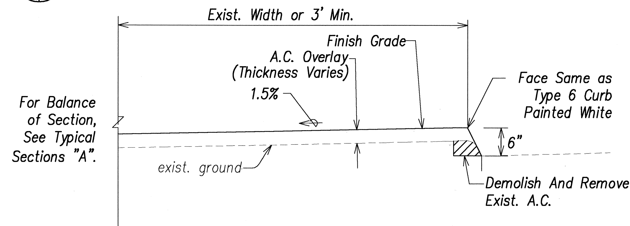
Various 47 TYPICAL SECTIONS - SHOULDER RECONSTRUCTION SCALE: 1" = 1'-0"
