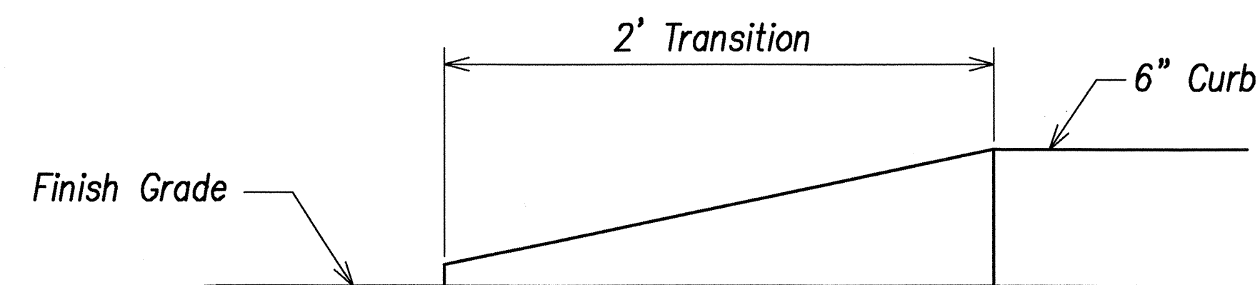
PROFILE: CURB TRANSITION SCALE: 1" = 0'-6" Various 64
