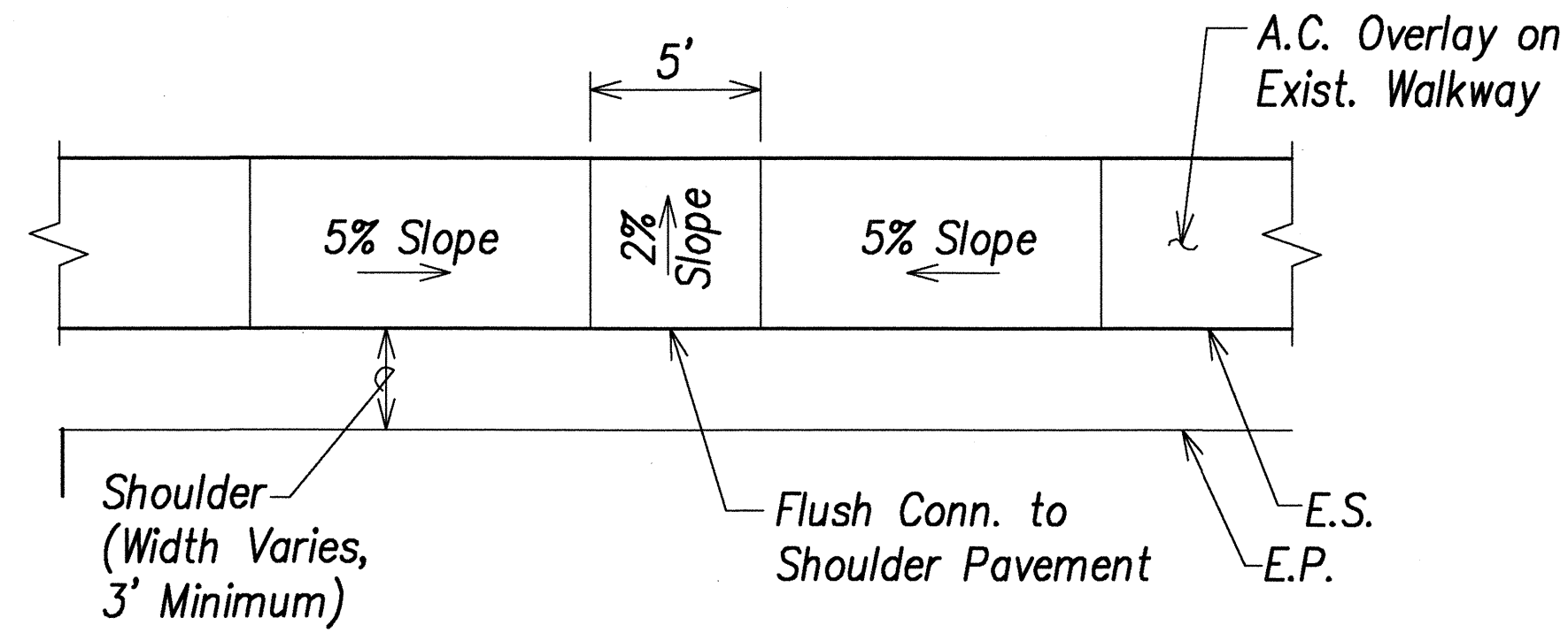
PASSING SPACE AT DRAIN OPENING SCALE: 1" = 5' Various 1/64
