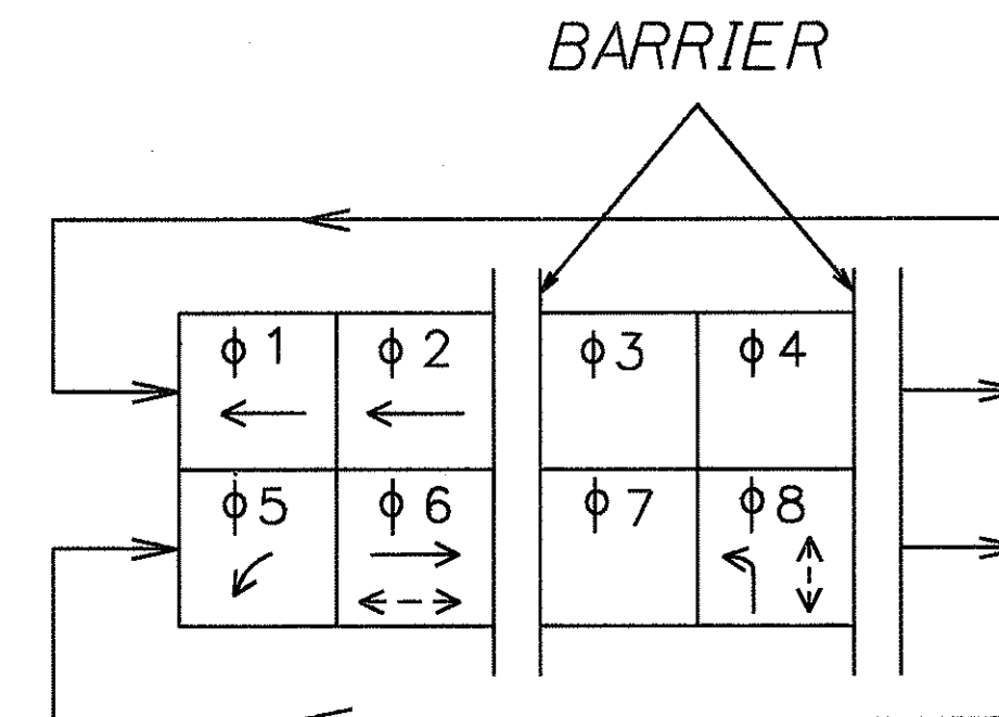
EXISTING PHASE DIAGRAM
