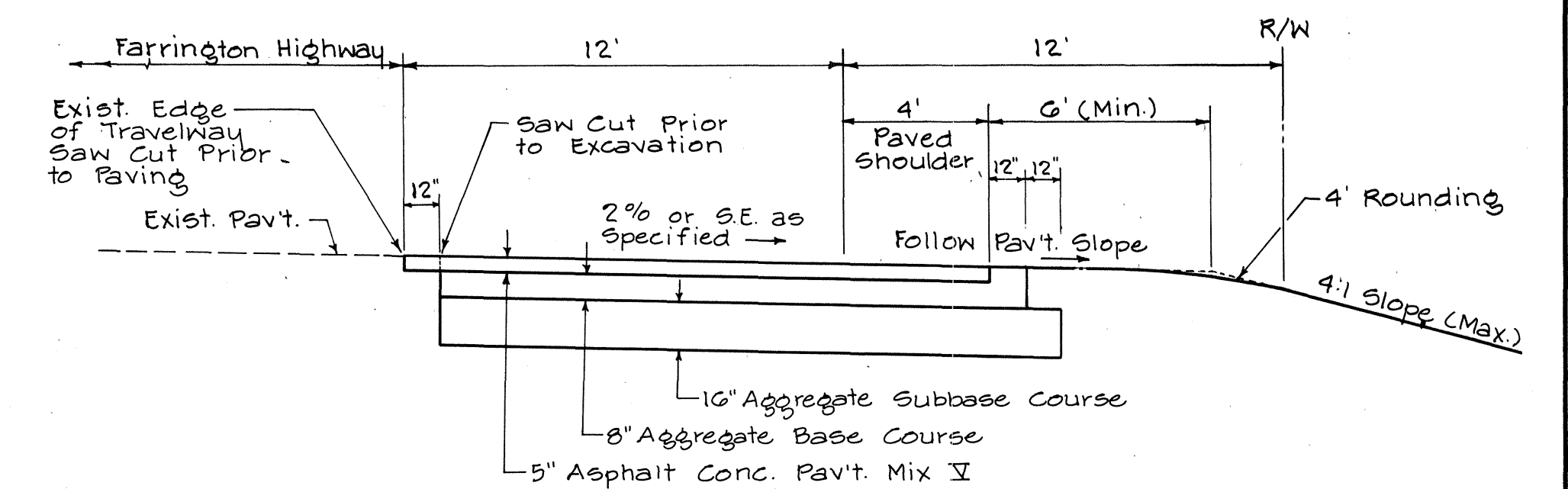
ROAD SECTION Decel. Lane Farrington Highway Sta. 99+44 to Sta. 105+84 Accel. Lane Farrington Highway Sta. 109+40 to Sta. 112+03 Scale: 1" = 4'
