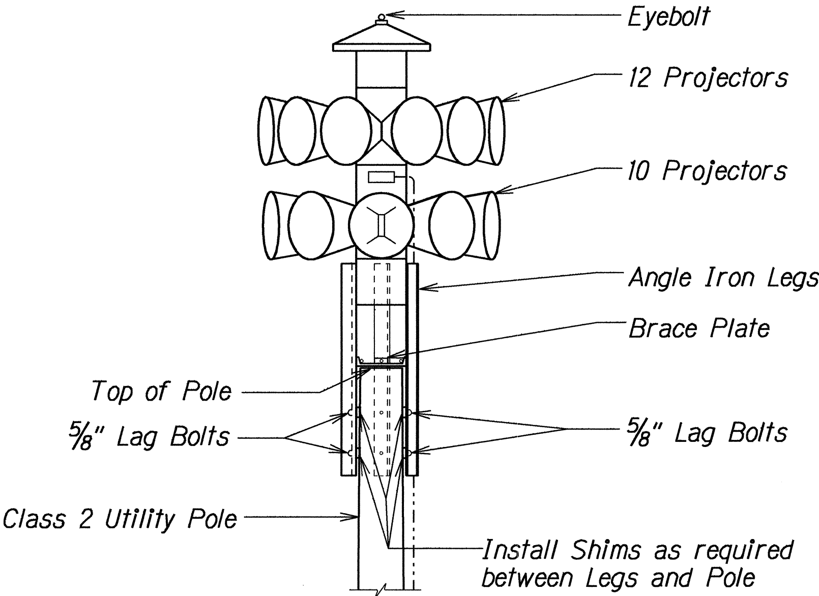
SIREN MOUNTING DETAIL Not to Scale
