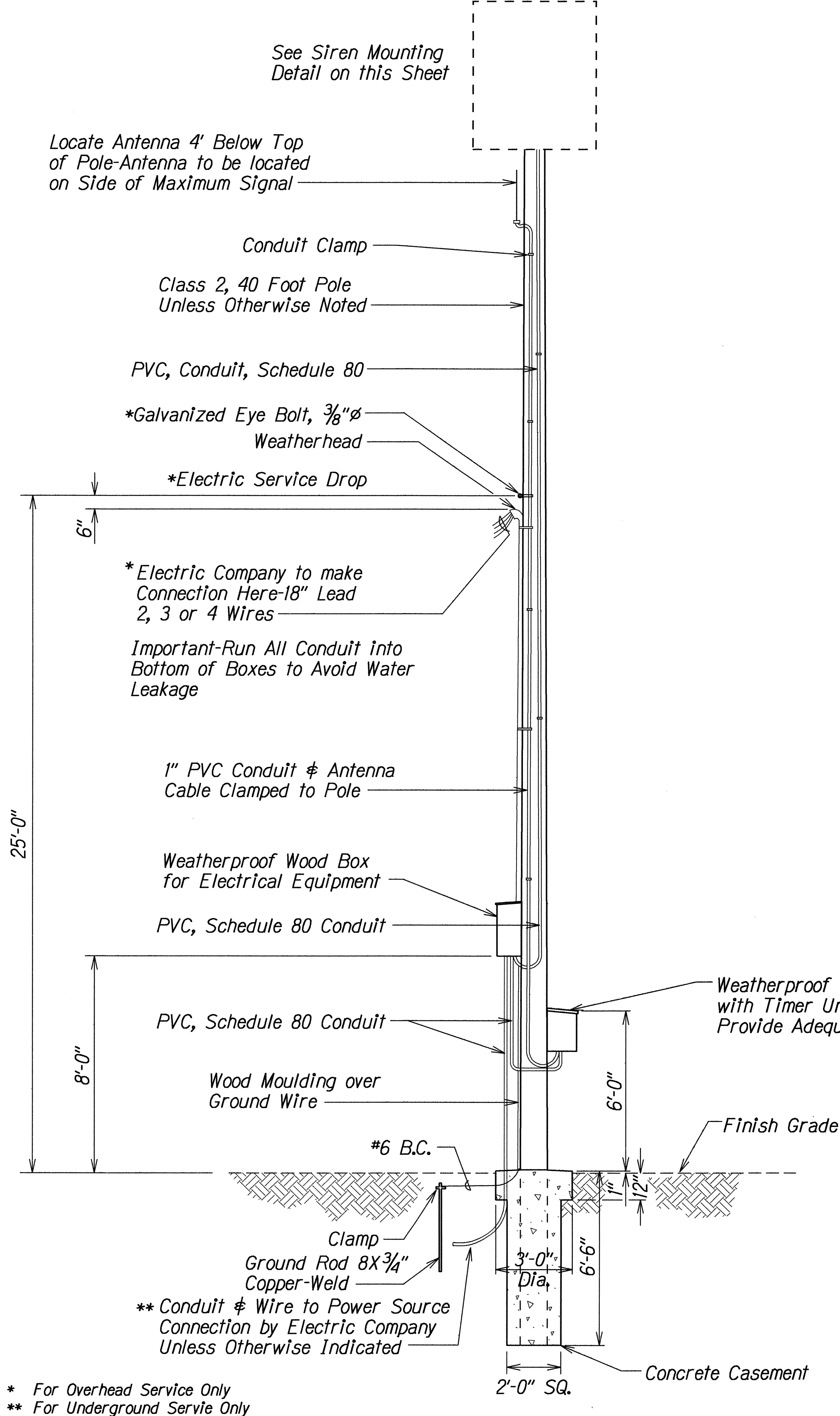
POLE DETAILS Not to Scale
