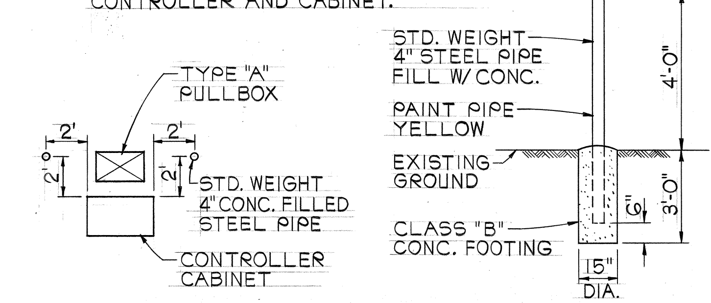
PLAN TYPE ELEVATION PIPE GUARD DETAIL NOT TO SCALE
