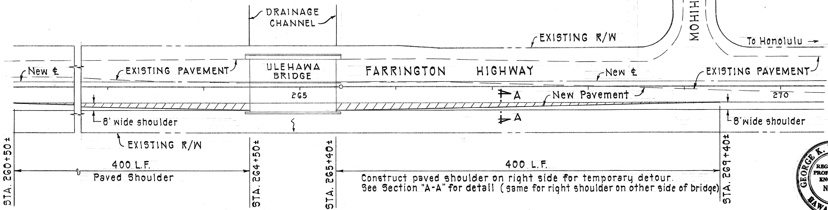
PLAN OF TEMPORARY DETOUR AT ULEHAWA BRIDGE
