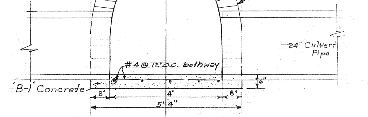
DETAIL-TYPE D DRAIN MANHOLE
