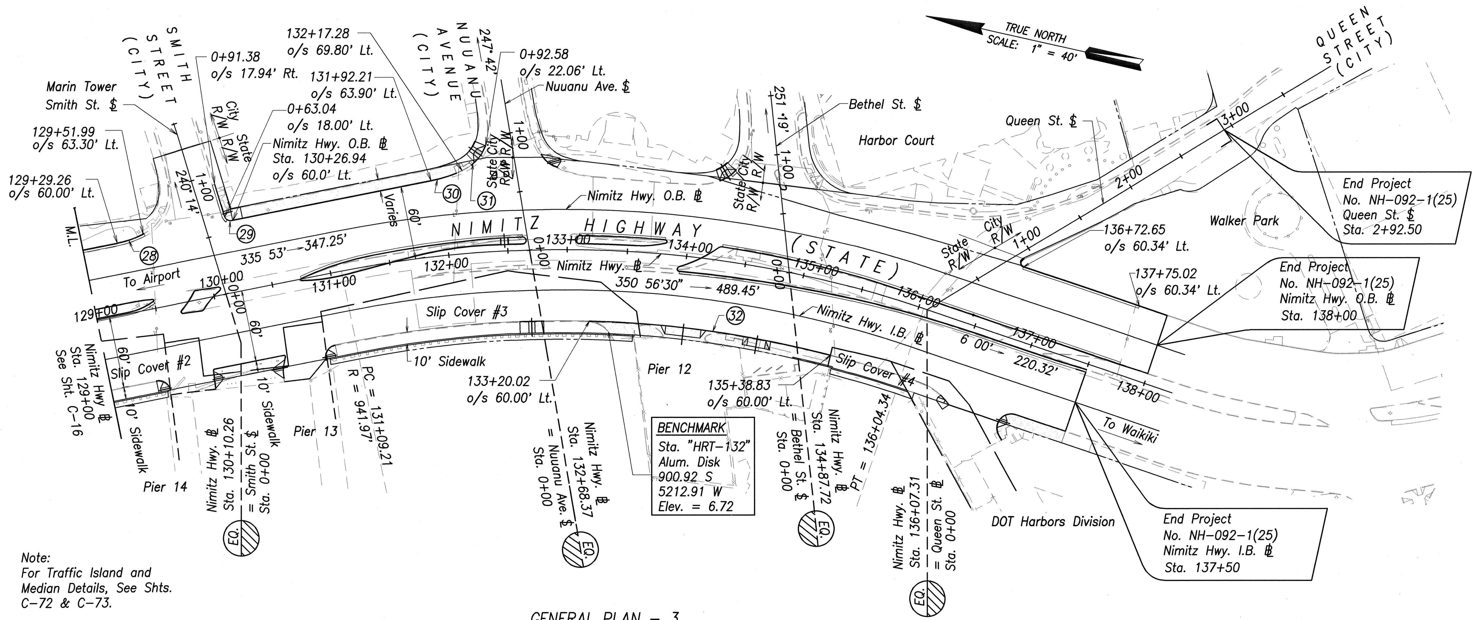
GENERAL PLAN - 3 Scale: 1" = 40'
