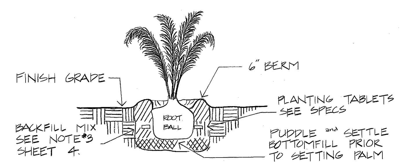
D PALM PLANTING DETAIL 6 NO SCALE
