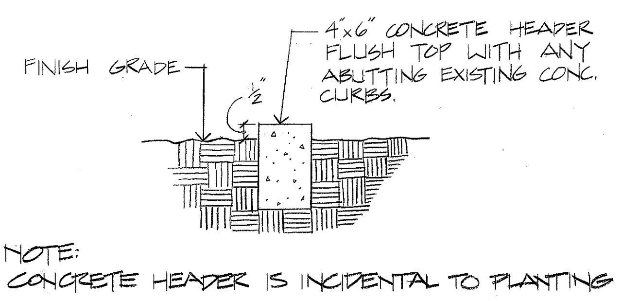
E CONCRETE HEADER DETAIL 7 NO SCALE
