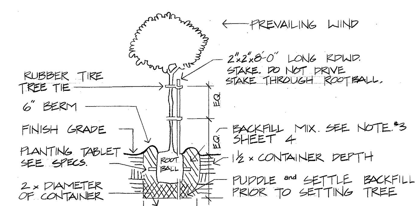
B TREE PLANTING and STAKING DETAIL 6 NO SCALE
