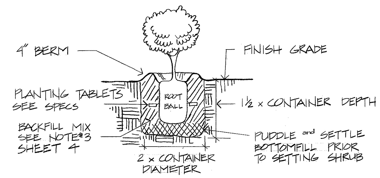
A SHRUB PLANTING DETAIL 6 NO SCALE
