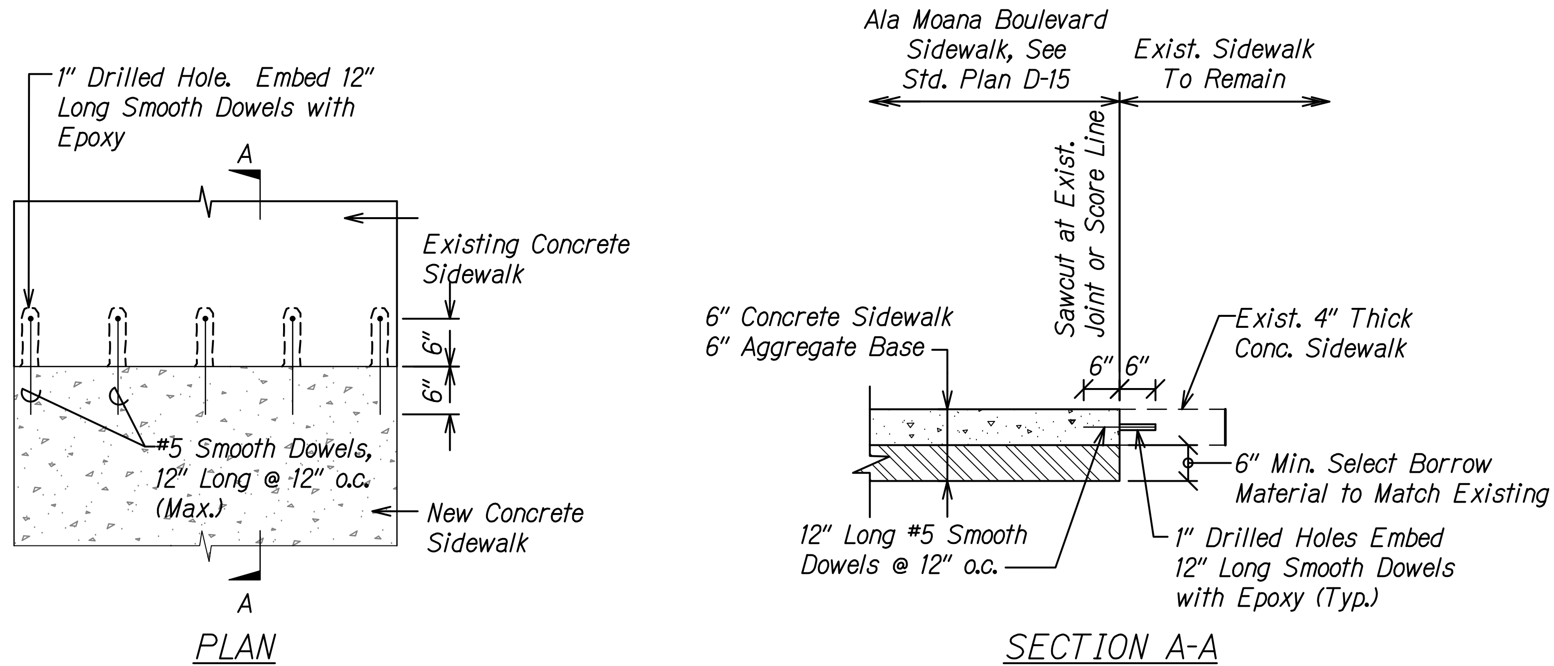
ALA MOANA BOULEVARD SIDEWALK CONNECTION DETAIL SCALE: 3/4" = 1'-0"
