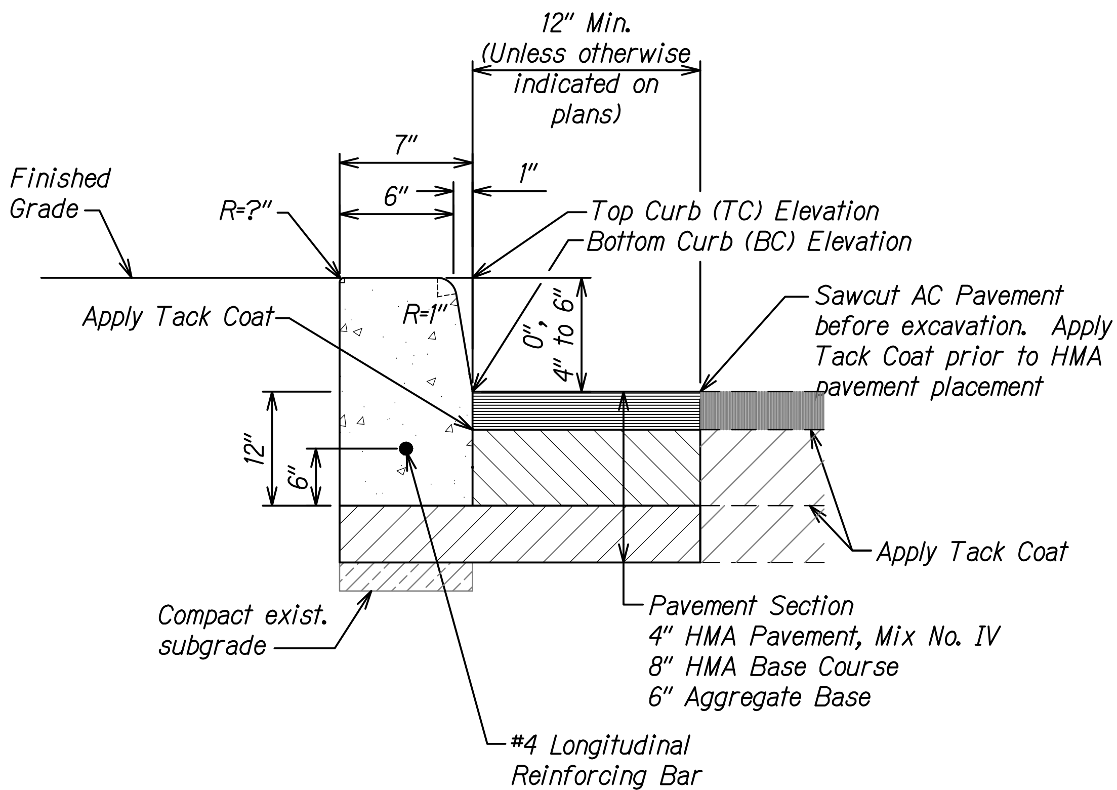
CURB, TYPE 2D MODIFIED NOT TO SCALE
