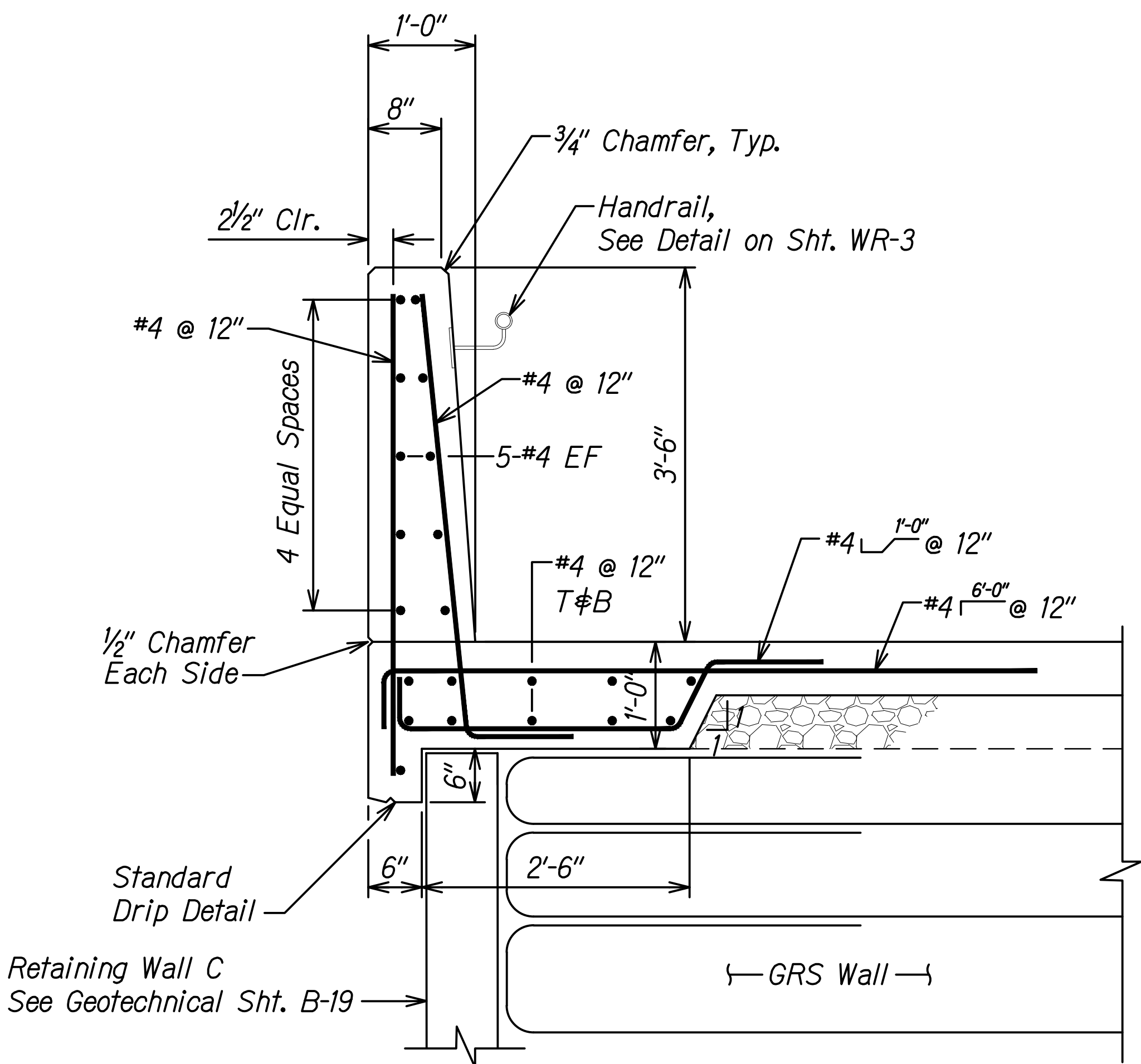
RETAINING WALL C CONCRETE RAILING DETAIL Not to Scale
