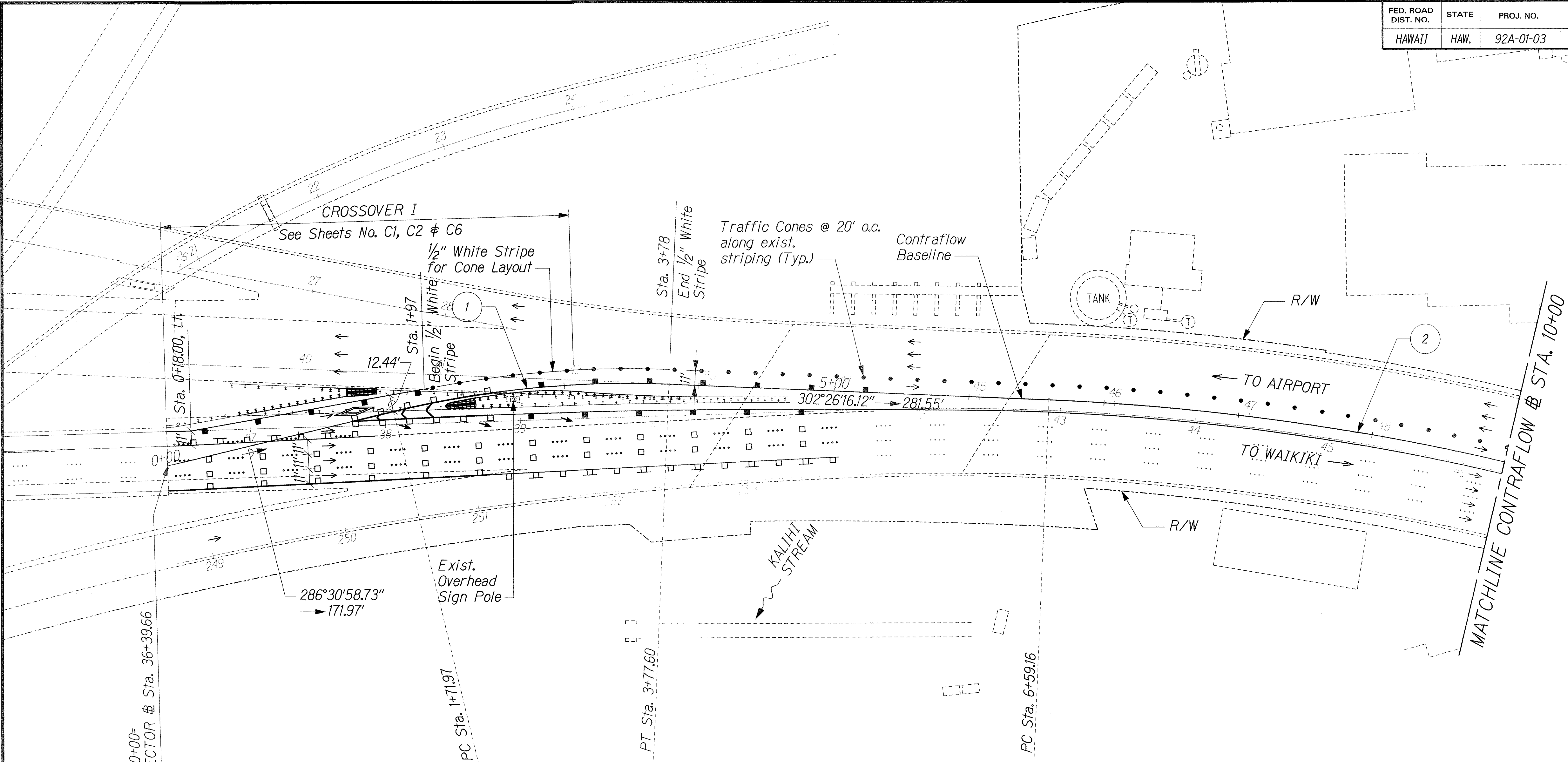
CONTRAFLOW CURVE DATA
