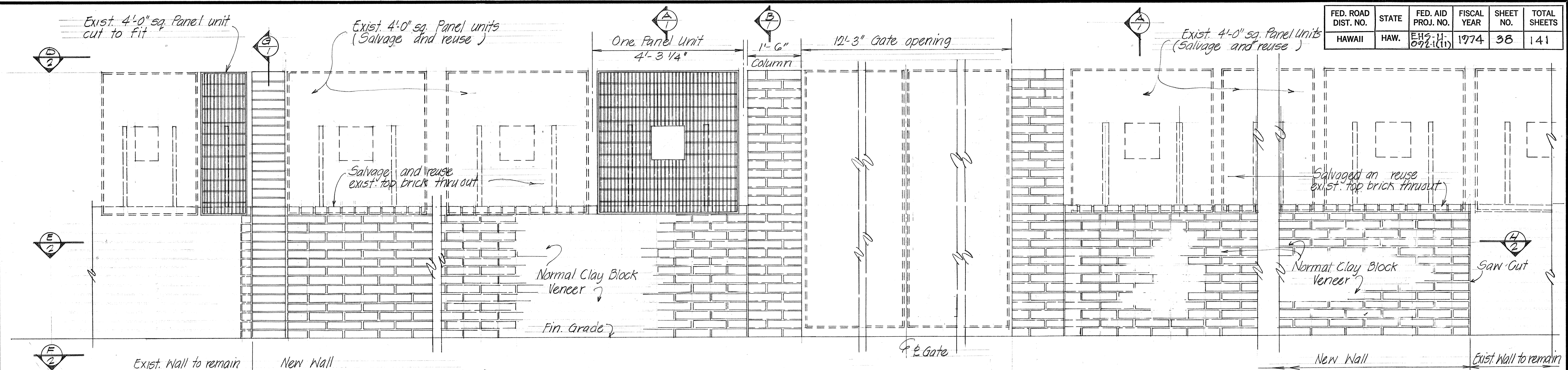
TYP WALL FENCE & GATE ELEVATION
