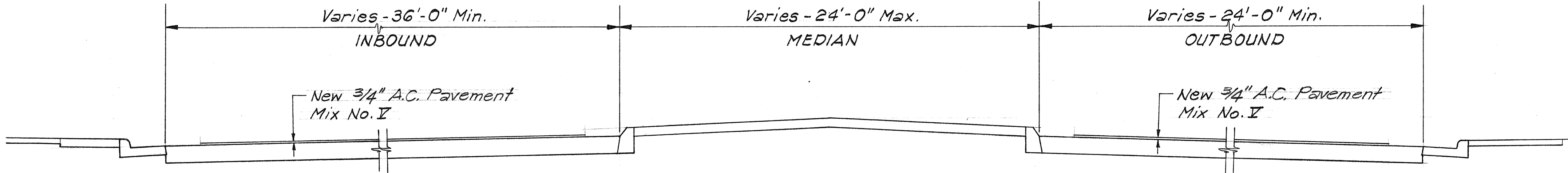
TYPICAL SECTION Scale: 1/4" = 1'-0"
