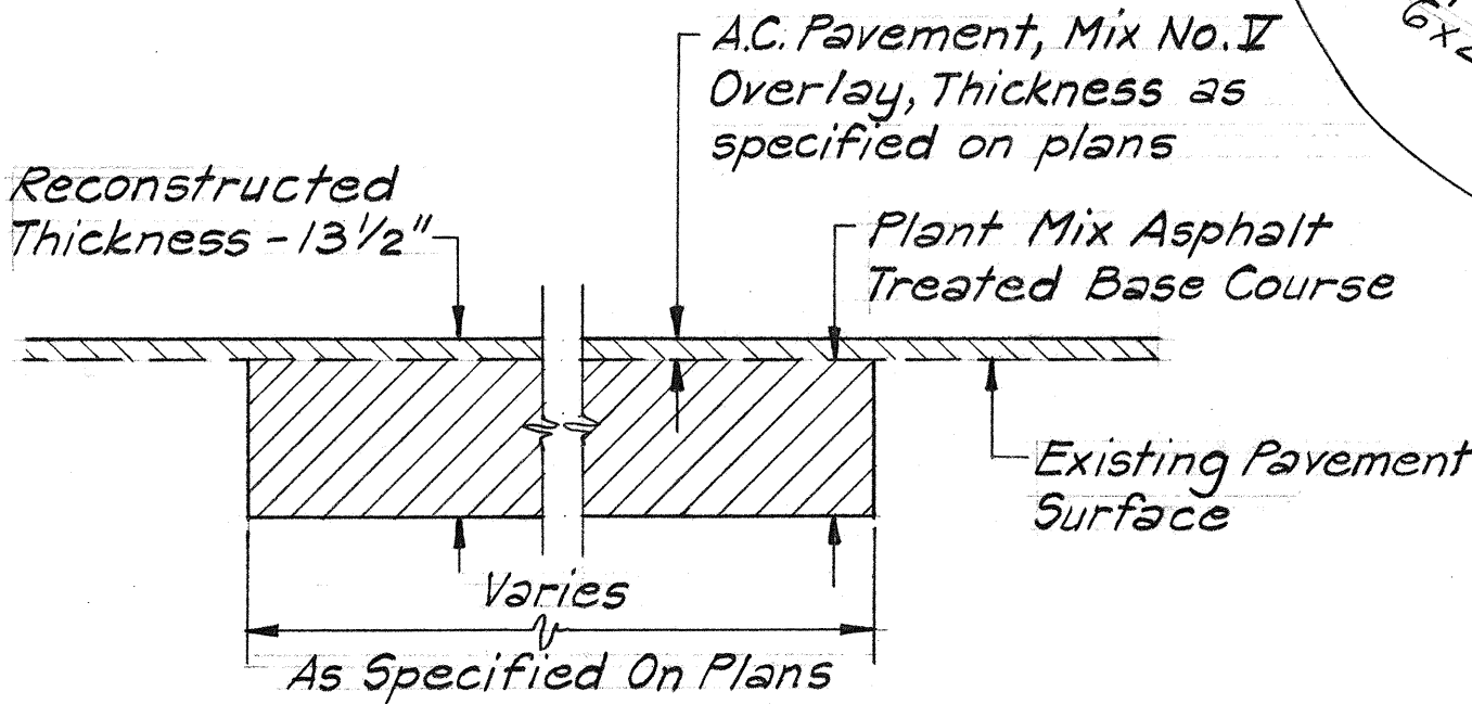
TYPICAL SECTION-RECONSTRUCTED AREA Scale: 3/4" = 1'-0"
