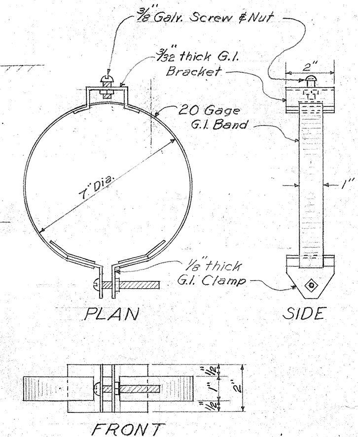
DETAIL OF ADJUSTABLE BAND BRACKET FOR SUPPORTING TRAFFIC SIGNS ON MONOTUBE LIGHTING STANDARDS
