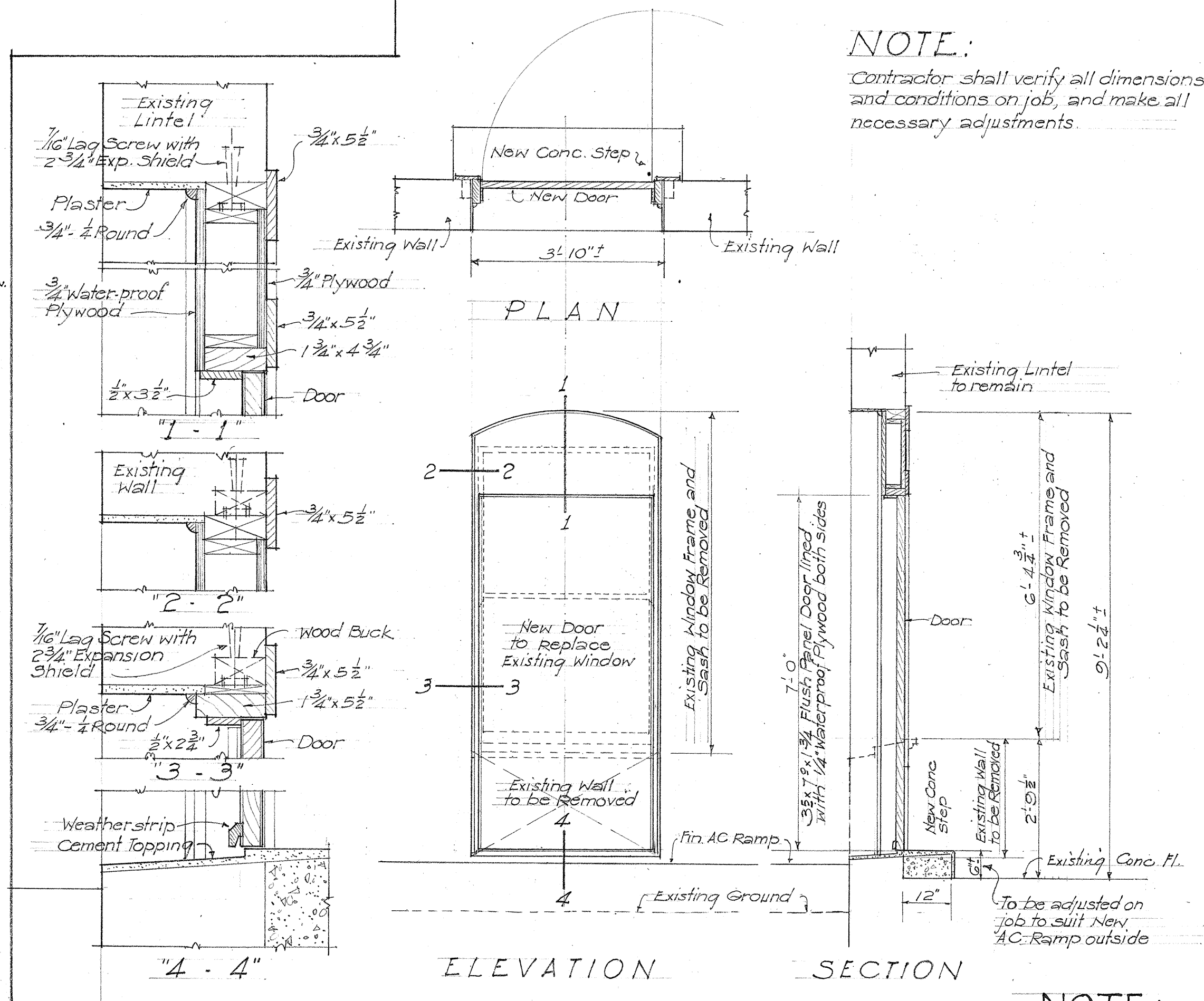
DOOR "A" EXISTING WINDOW TO BE REPLACED WITH NEW DOOR Scale: 1/2" = 1'-0"
