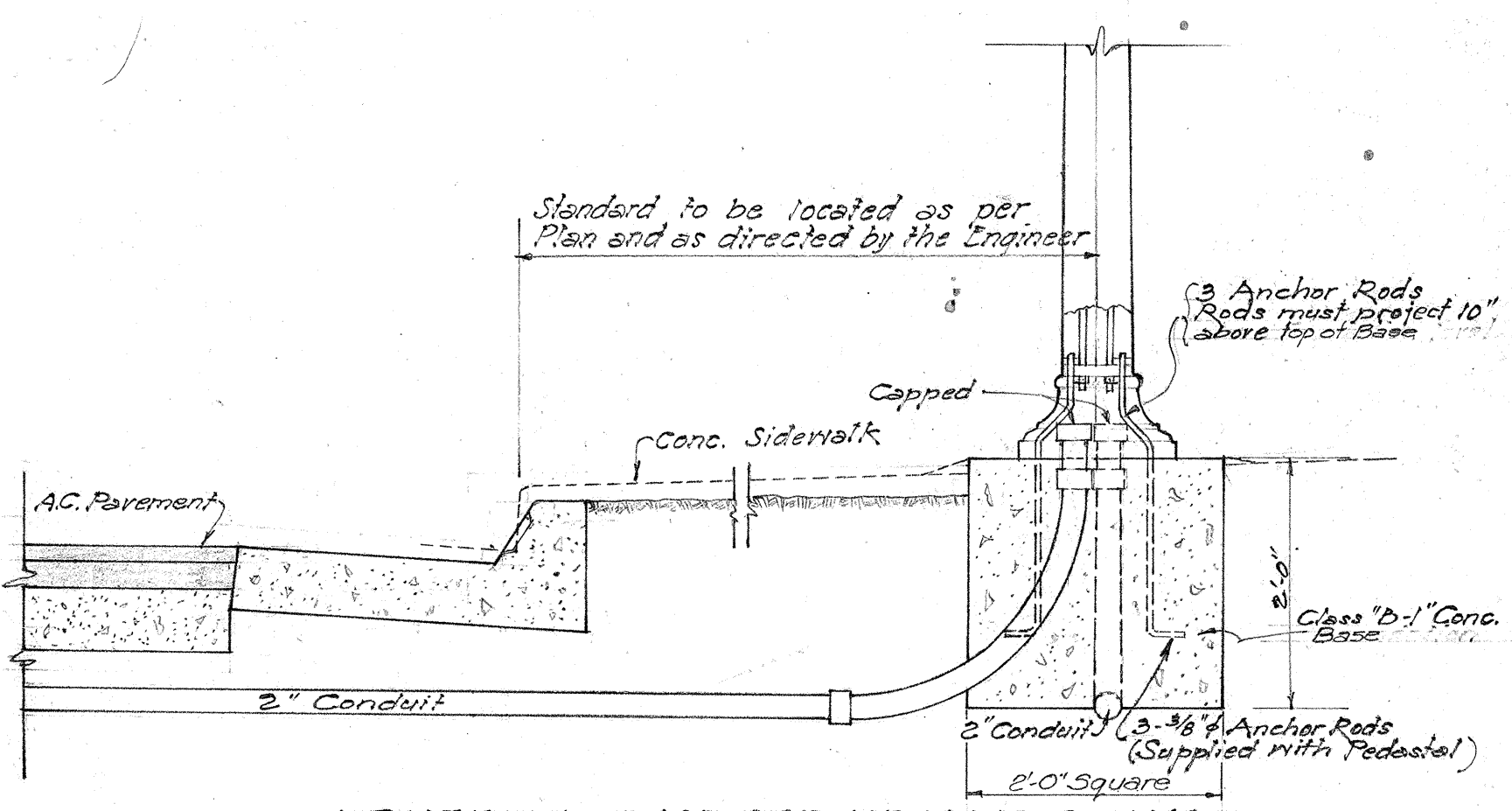
CONCRETE BASE FOR TRAFFIC SIGNAL STANDARD AND DISPATCHER CABINET STANDARD Scale: 3/4" = 1'-0"
