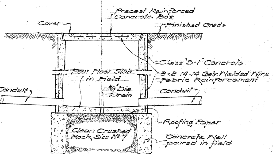
SECTION "A-A" DETAIL OF PULL BOX TYPE "A" Scale: 1" = 1'-0"
