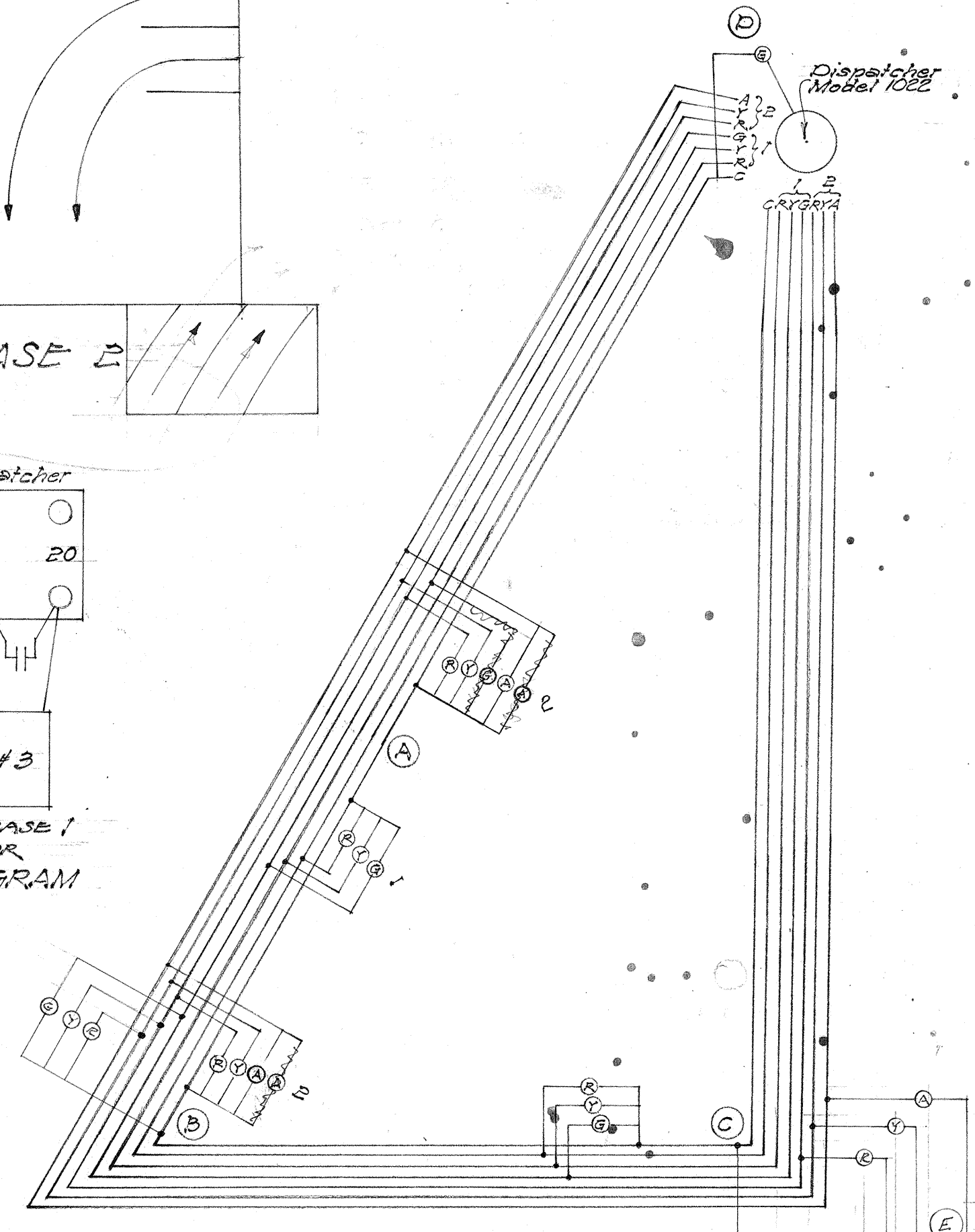
GEOGRAPHICAL CIRCUIT WIRING DIAGRAM Not to Scale
