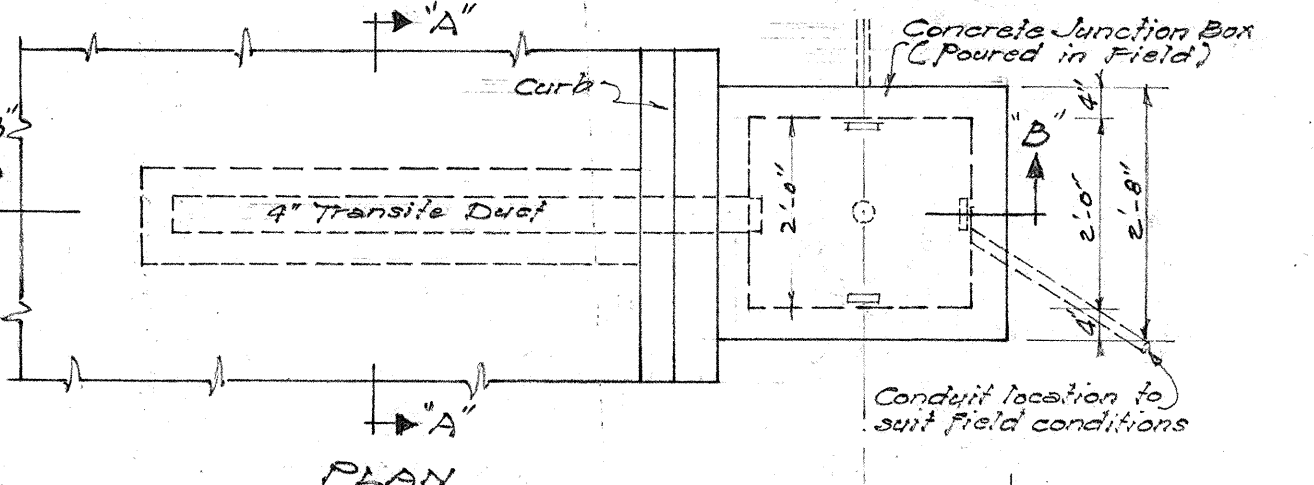
SECTION "B-B" TYPICAL ROAD SECTION SHOWING TRAFFIC DETECTOR JUNCTION BOX AND DUCT Scale: 1/2" = 1'-0"
