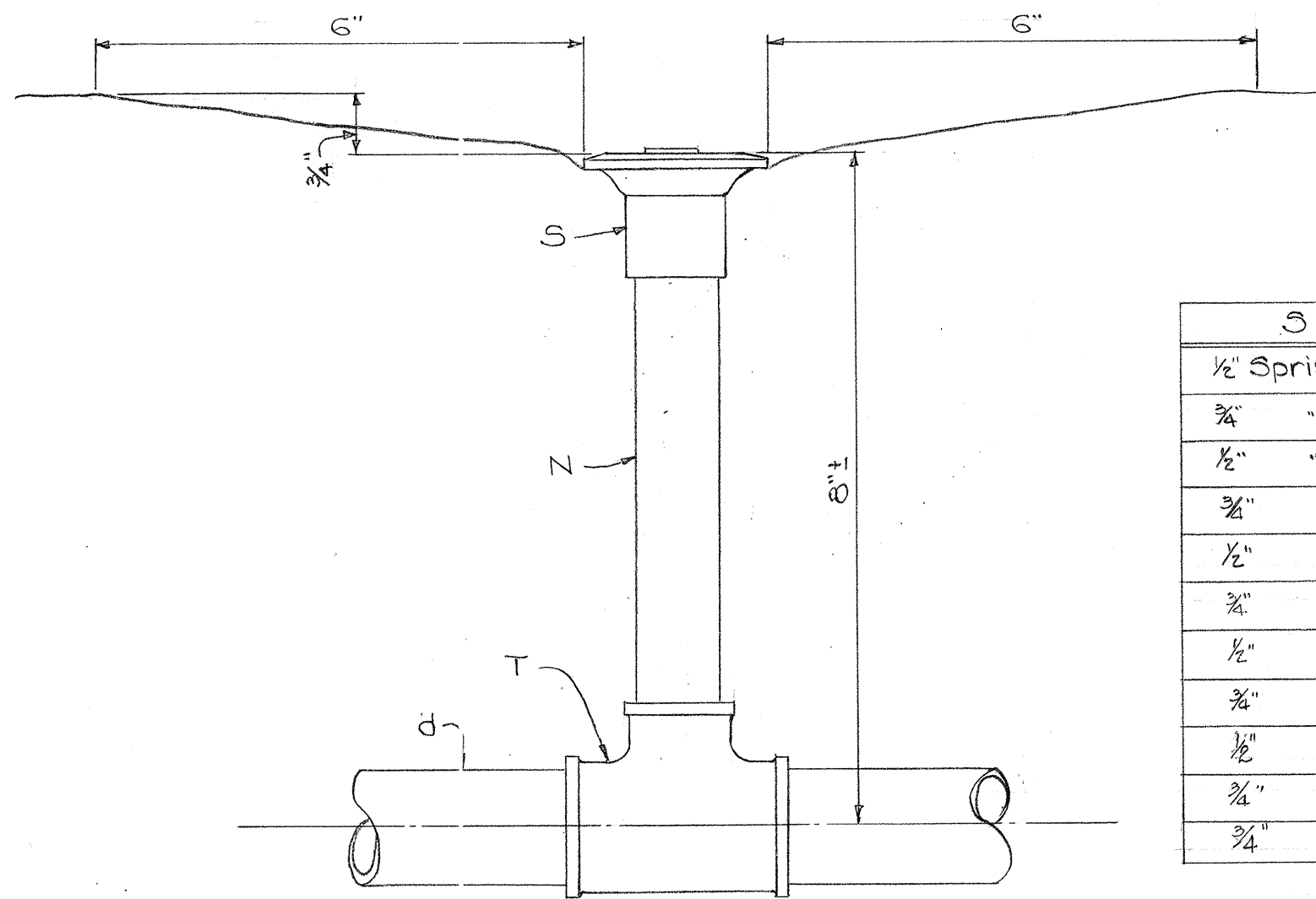
DETAIL "M" CONNECTION OF SPRINKLERS TO FEEDER PIPES
