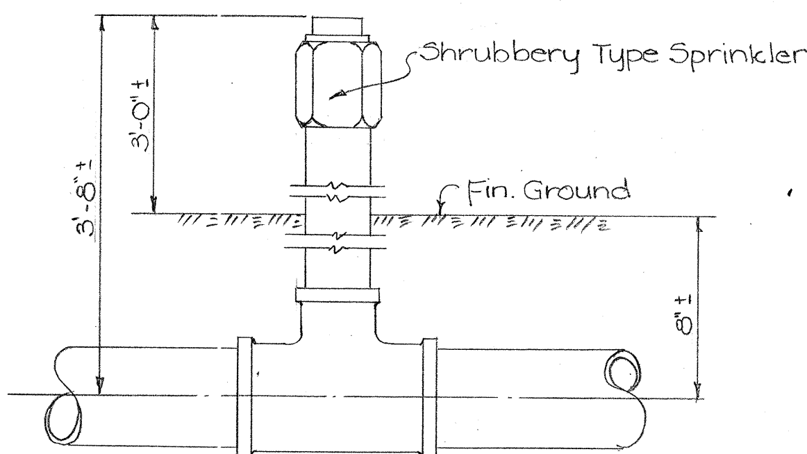
DETAIL "N" CONNECTION OF SHRUBBERY TYPE SPRINKLER HEADS TO FEEDER PIPES
