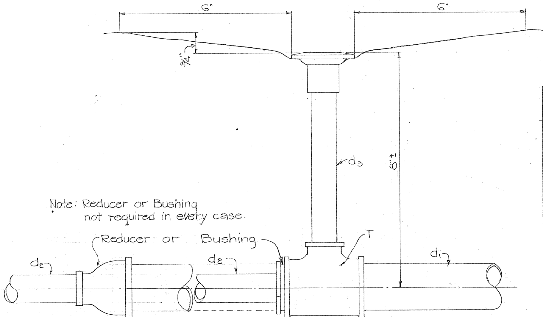
DETAIL "P" CONNECTION OF A LARGE PIPE, A SMALLER PIPE AND SPRINKLER HEAD
