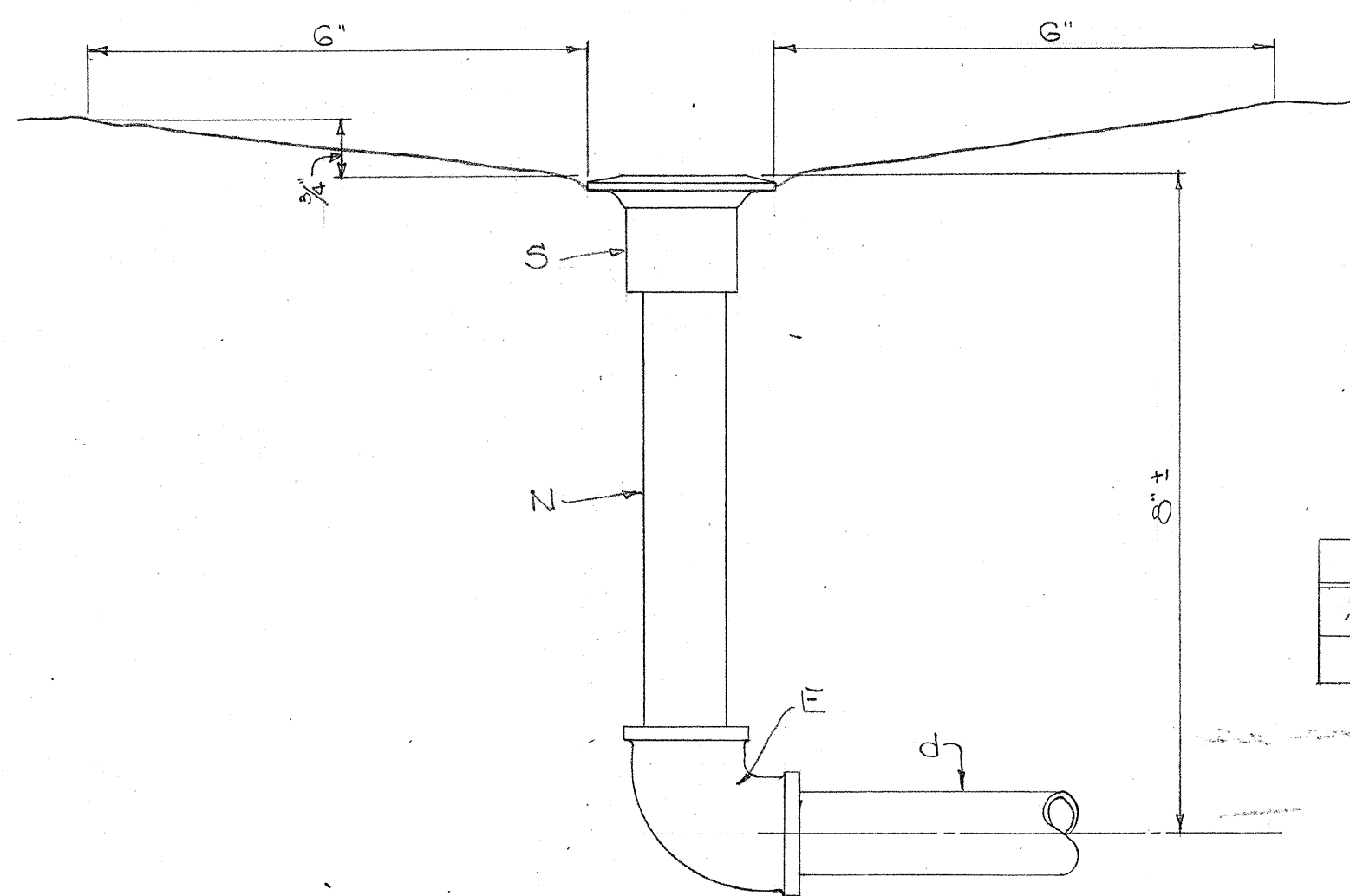
DETAIL "Q" CONNECTION OF SPRINKLER HEADS AT ENDS OF PIPES
