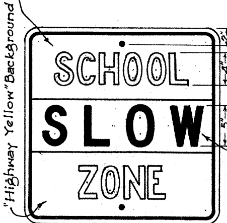
R-41-S 24" x 24"
