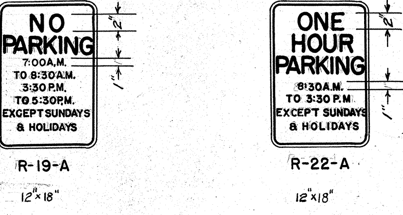
REGULATORY SIGNS R-25-A, R-19-A Red letters, and numerals and white background R-22-A Green letters and numerals and white background Scale: 1" = 1'-0"
