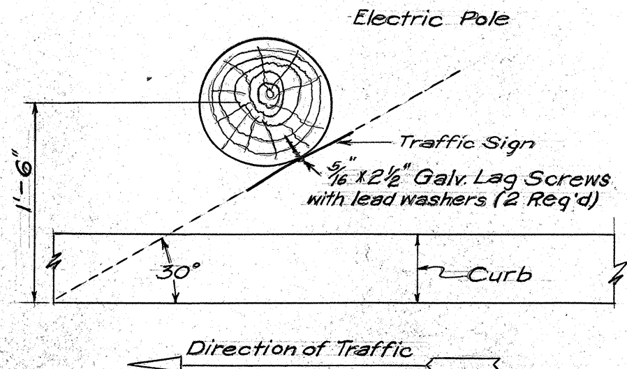
DETAIL SHOWING ANGLE OF TRAFFIC SIGNS AND CURB LINE Scale: 1" = 1'-0" (Above detail applies to signs "R-19-A" & "R-22-A" only)
