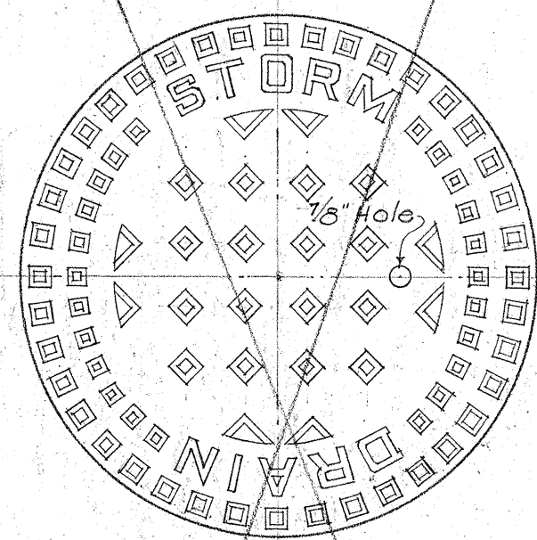
PLAN OF TOP OF COVER
