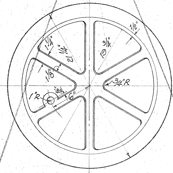
PLAN OF BOTTOM SCALE 1/2" = 1'-0"
