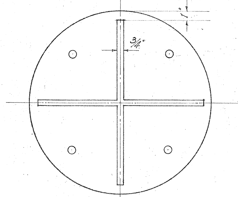
PLAN OF BOTTOM SCALE: 1/2" = 1'-0"
