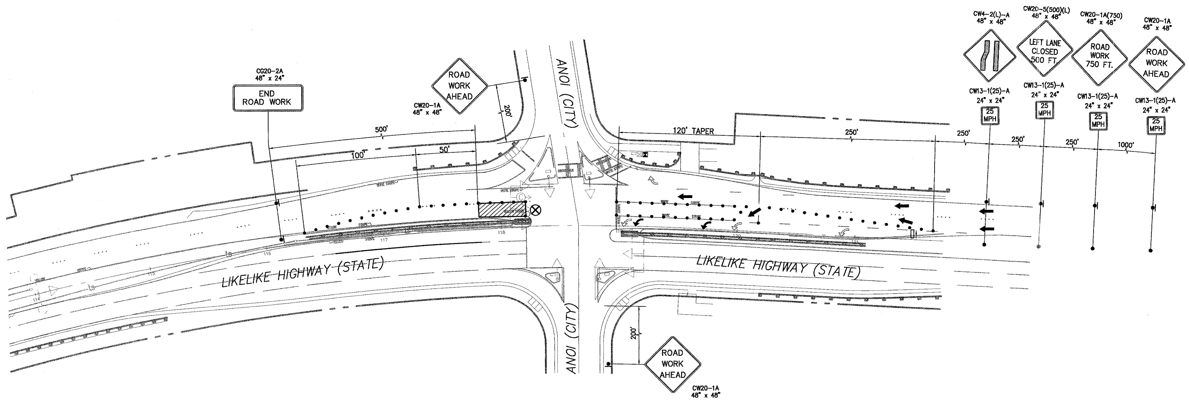
TRAFFIC CONTROL PLAN (LIKELIKE - ANOI INTERSECTION)-1
