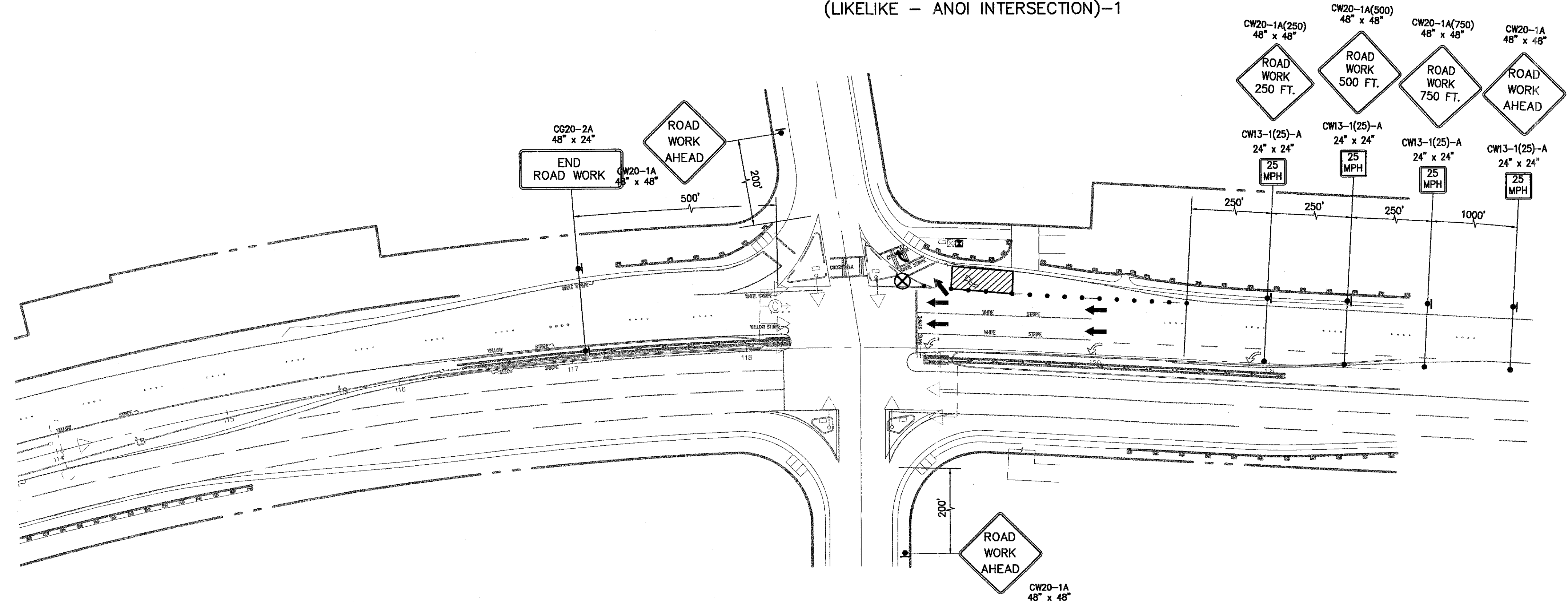
TRAFFIC CONTROL PLAN (LIKELIKE - ANOI INTERSECTION)-2
