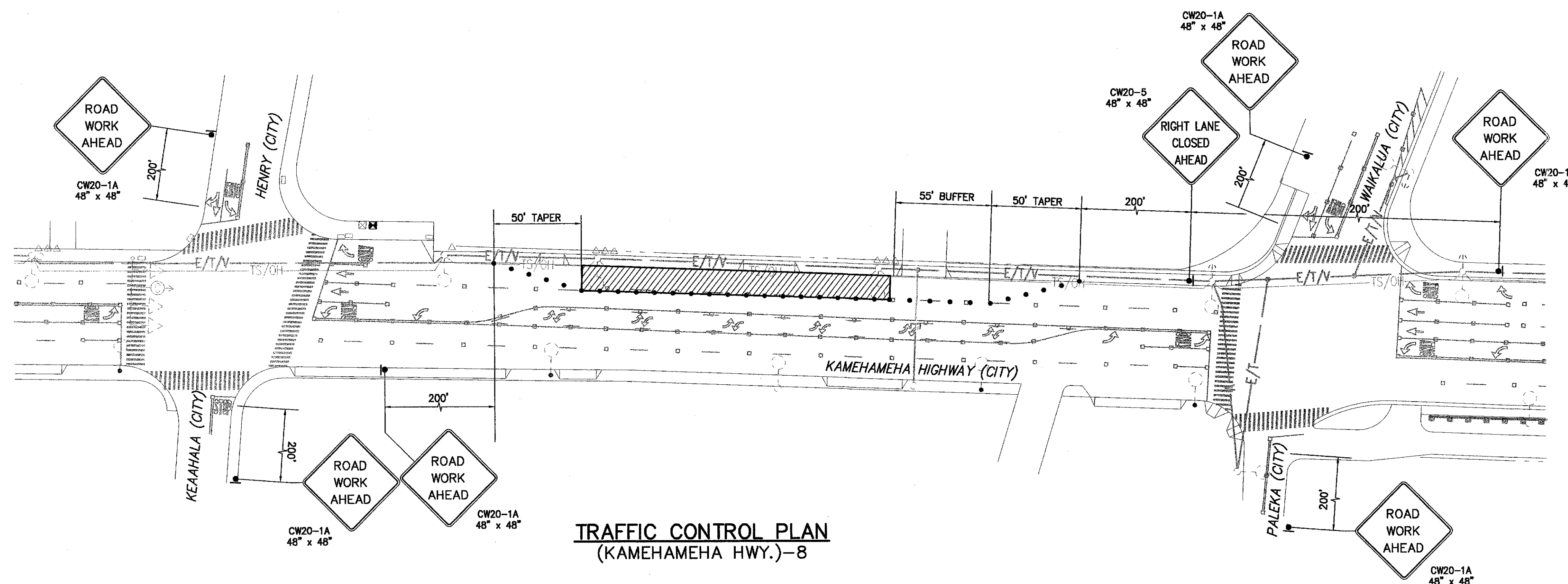
TRAFFIC CONTROL PLAN (KAMEHAMEHA HWY. / KEAAHALA INTERSECTION)
