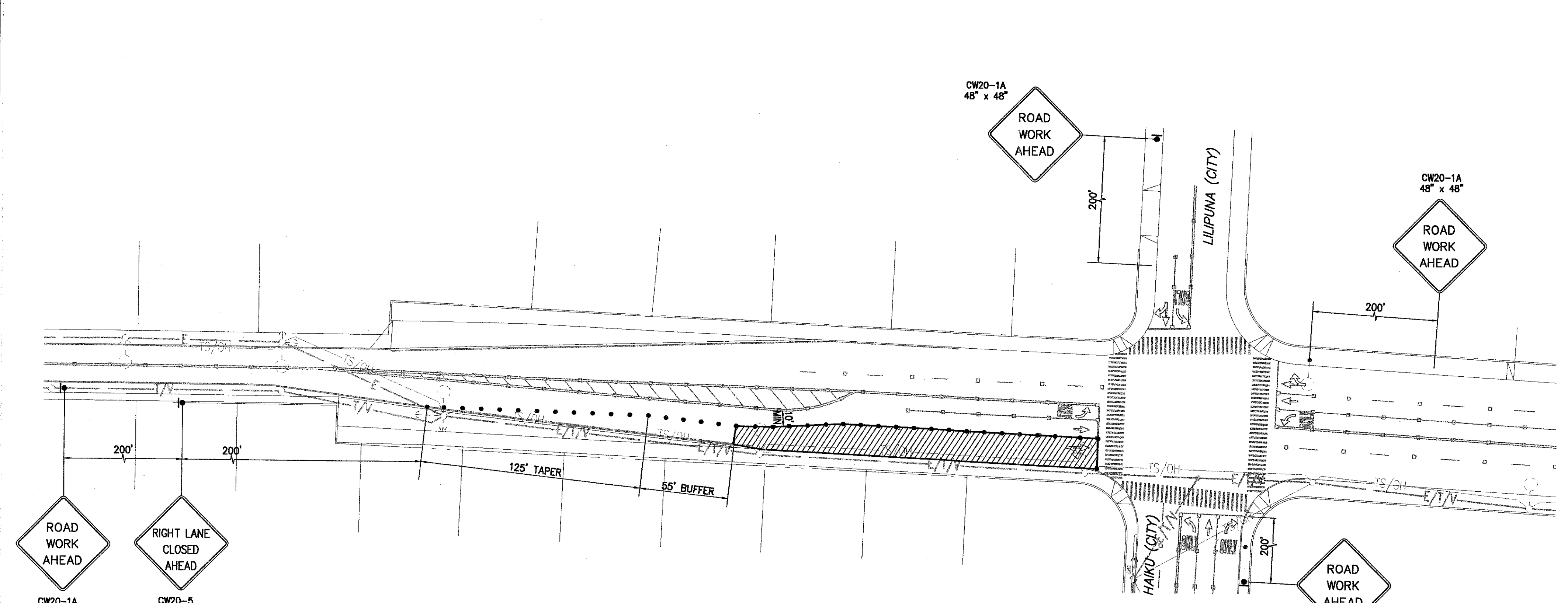
TRAFFIC CONTROL PLAN (KAMEHAMEHA HWY.)-4
