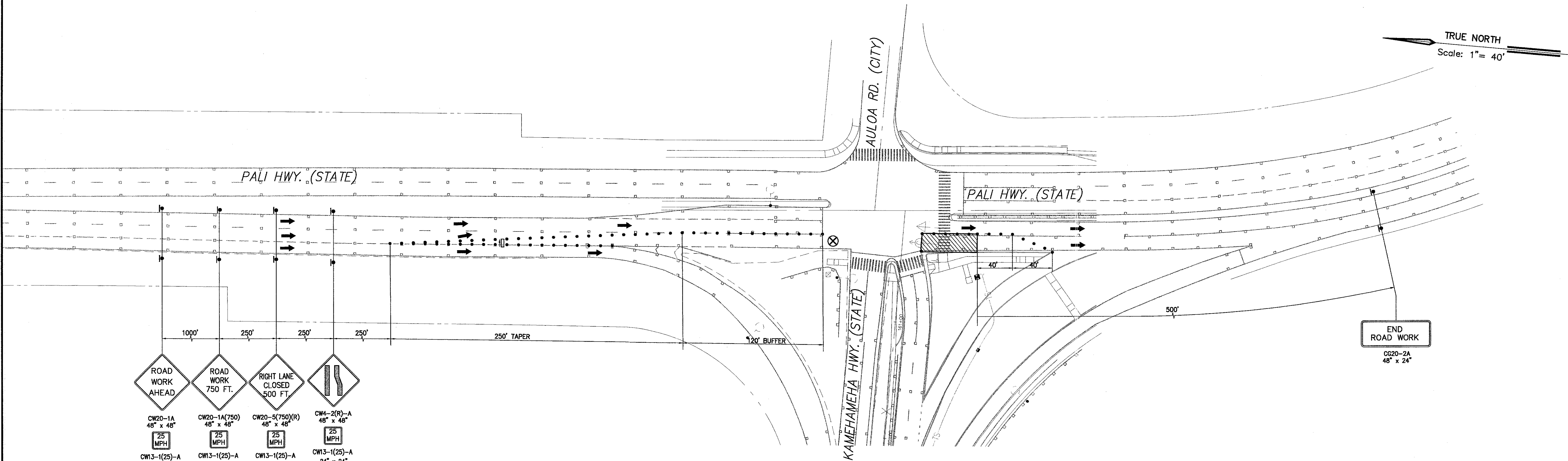
TRAFFIC CONTROL PLAN (KAMEHAMEHA HWY - PALI HWY. INTERSECTION)-3
