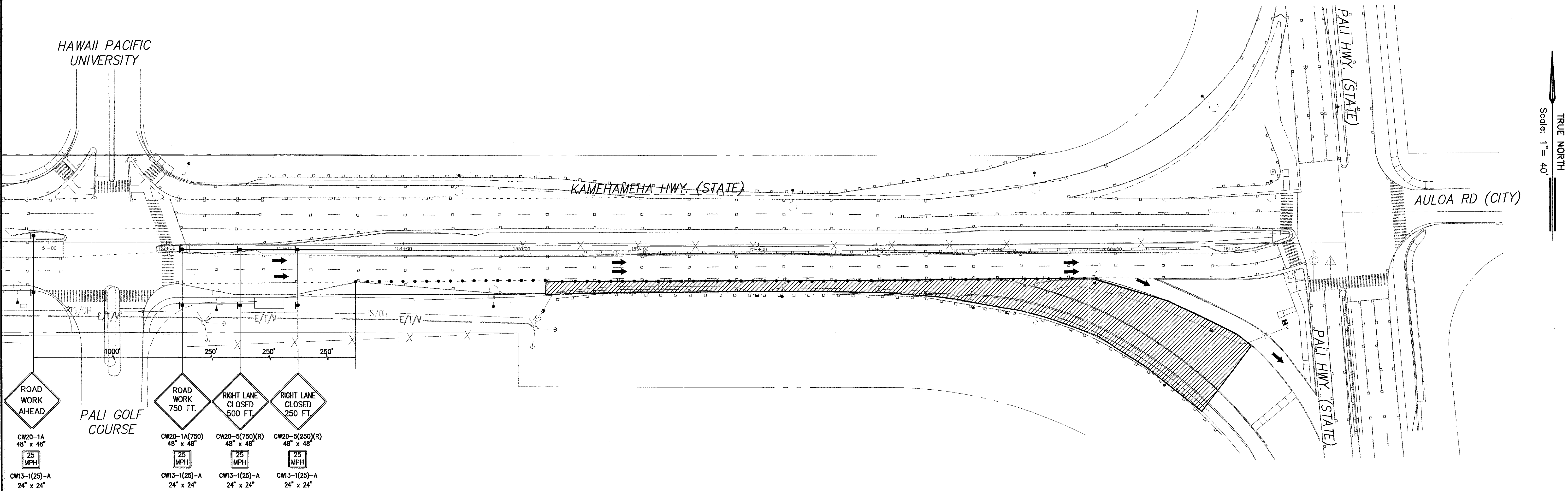
TRAFFIC CONTROL PLAN (KAMEHAMEHA HWY - PALI HWY. INTERSECTION)-1
