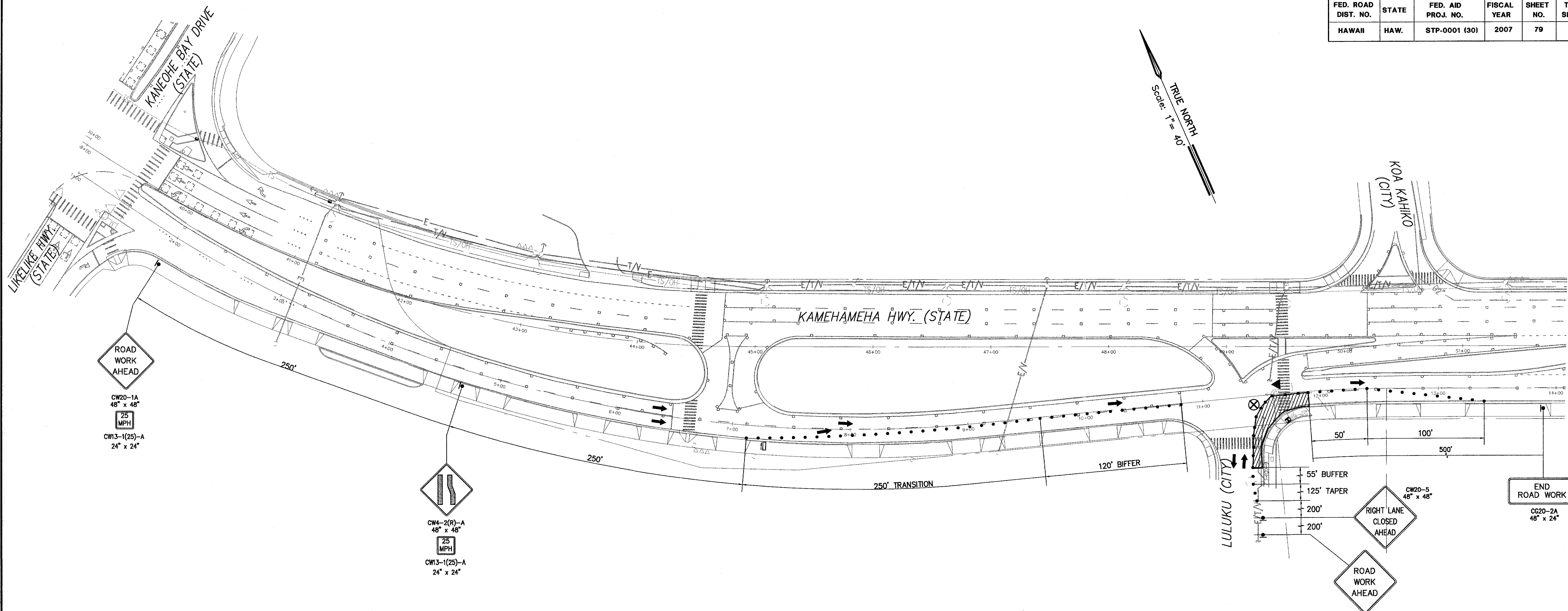
TRAFFIC CONTROL PLAN (KAMEHAMEHA - LULUKU INTERSECTION)
