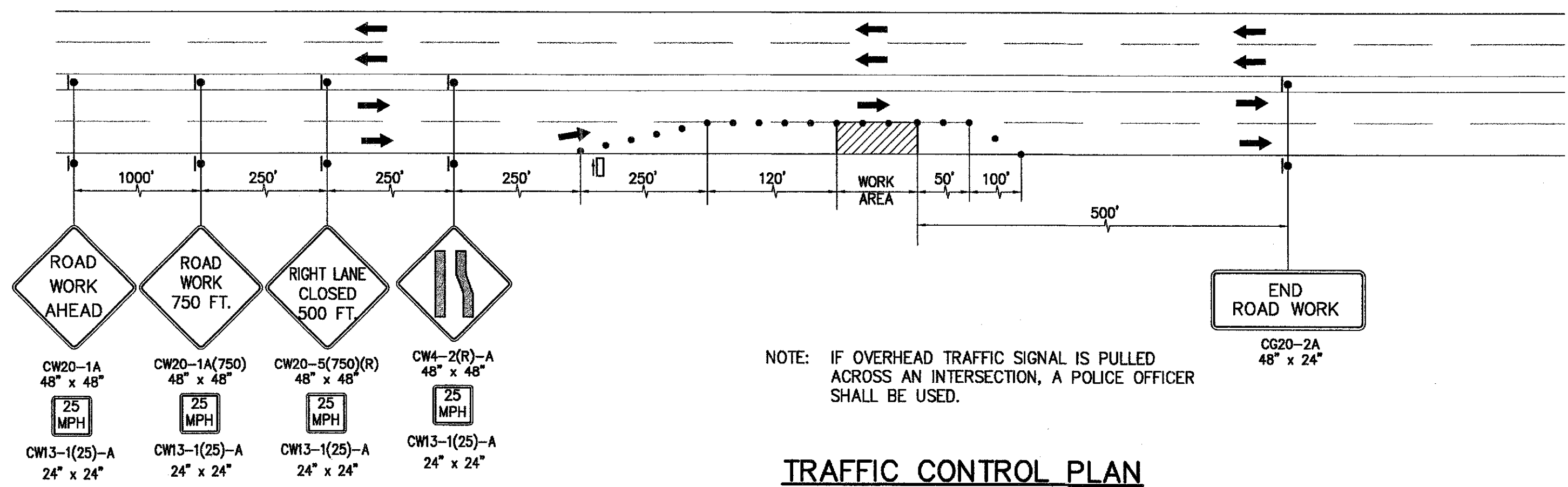
TRAFFIC CONTROL PLAN MULTILANE DIVIDED HIGHWAY - RIGHT LANE CLOSED KAMEHAMEHA HIGHWAY - MAKAI (Kaneohe Bay Dr. to ENTRANCE OF Kaneohe Elem.)
