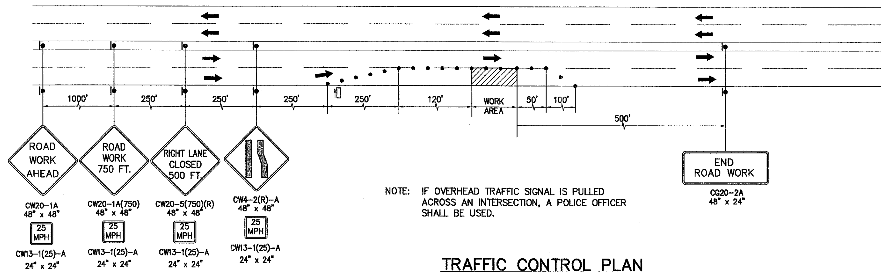
TRAFFIC CONTROL PLAN MULTILANE DIVIDED HIGHWAY - RIGHT LANE CLOSED KAMEHAMEHA HIGHWAY - MAUKA (KUU HOME TO PALI GOLF COURSE)
