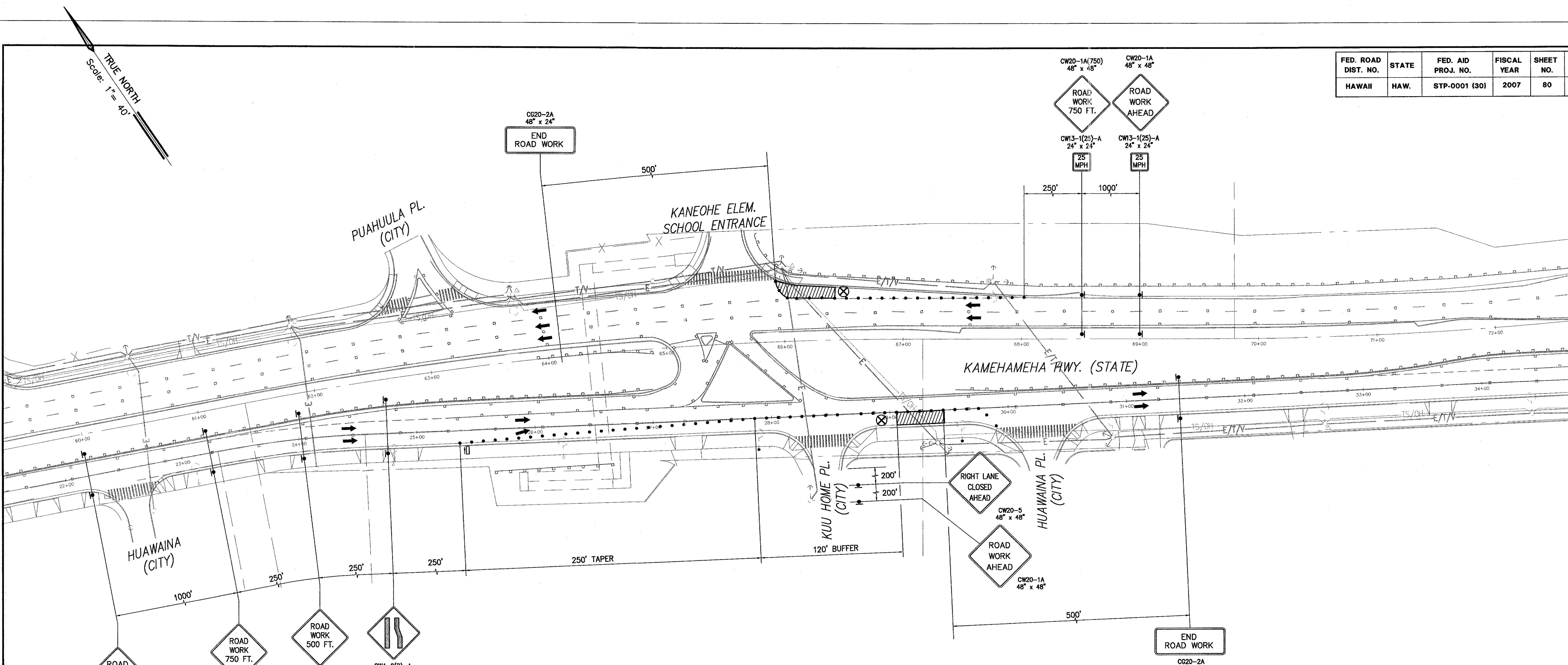
TRAFFIC CONTROL PLAN (KAMEHAMEHA - KUU HOME INTERSECTION)
