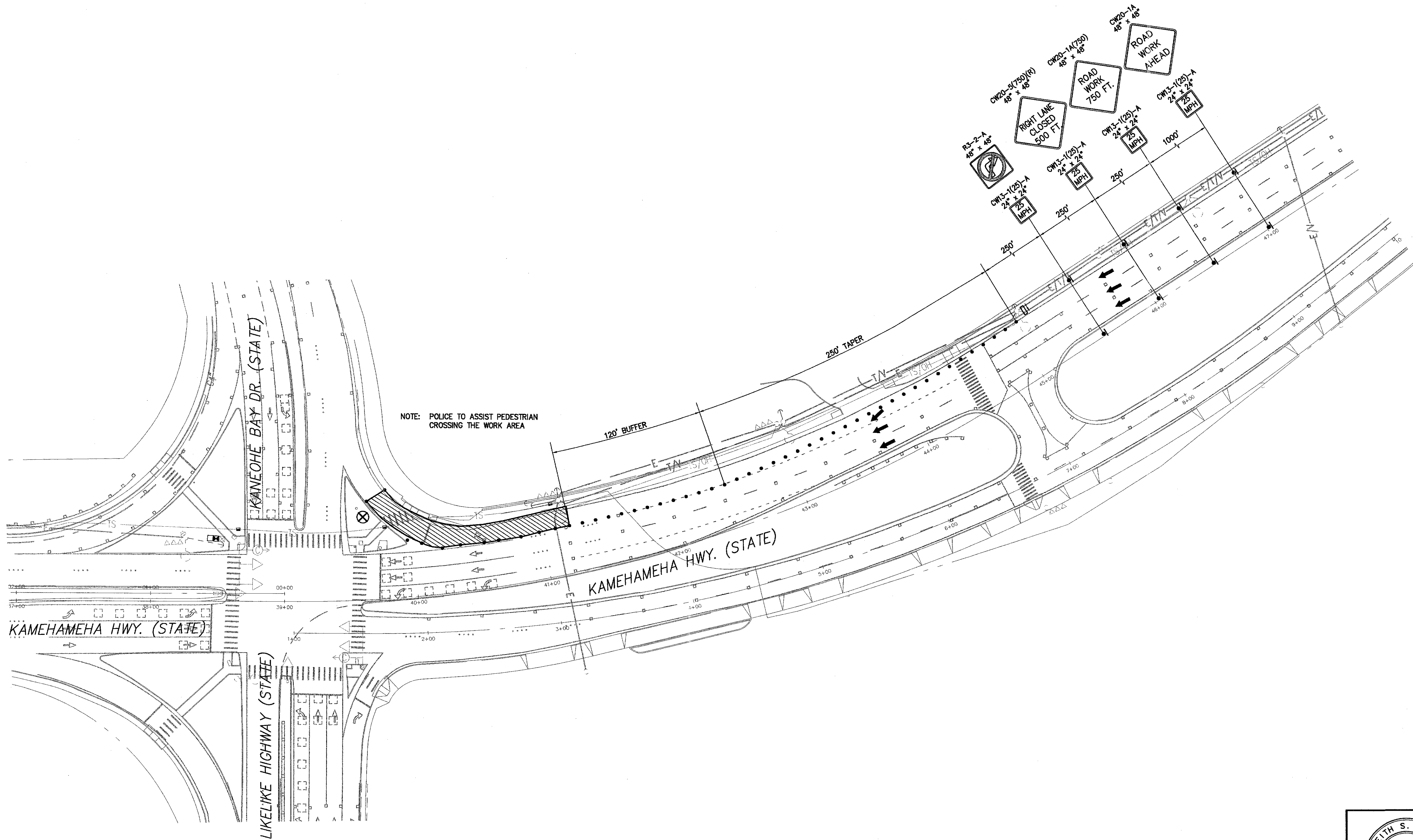
TRAFFIC CONTROL PLAN (KAMEHAMEHA - LIKELIKE INTERSECTION)-7
