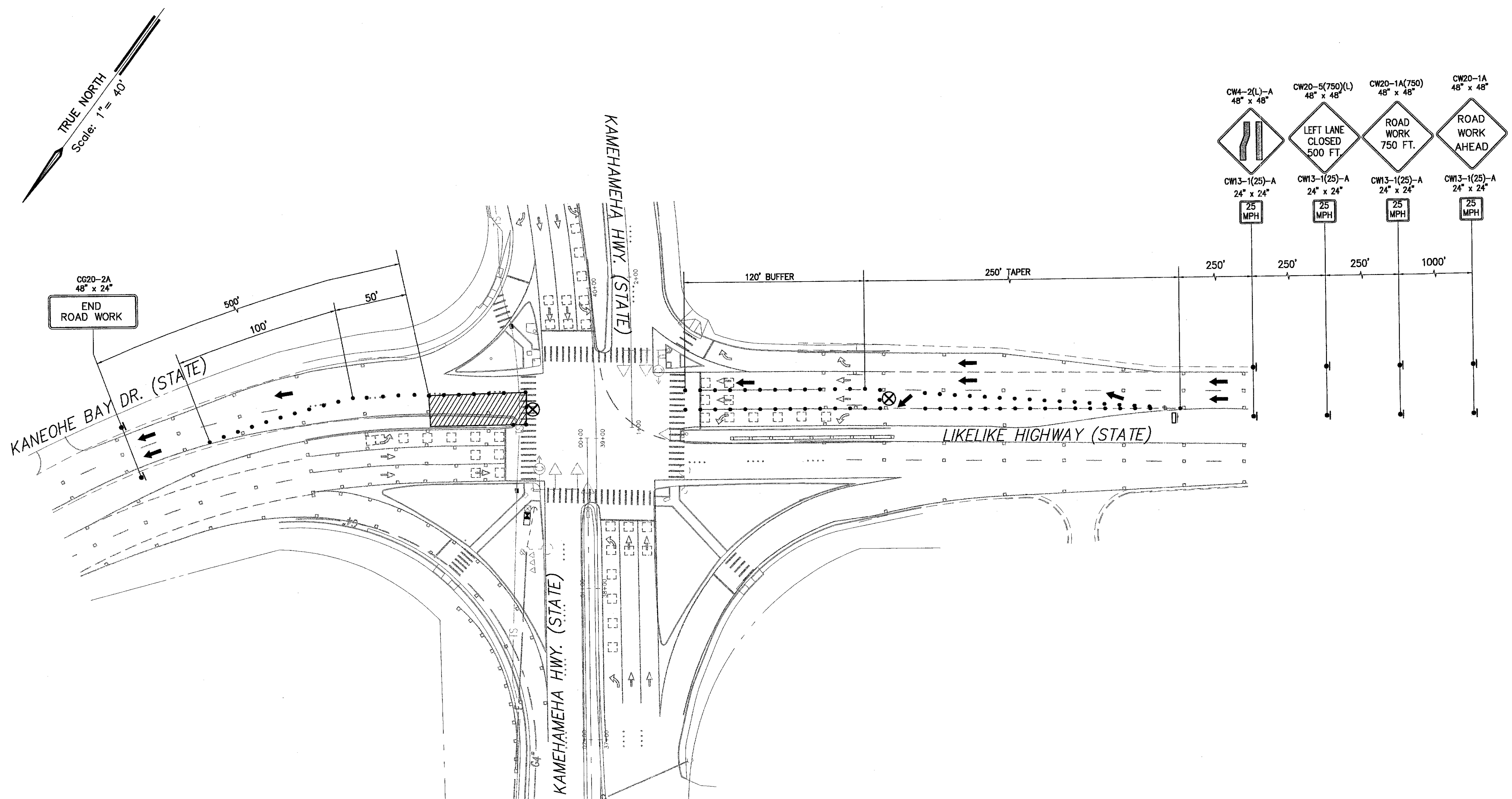
TRAFFIC CONTROL PLAN (KAMEHAMEHA - LIKELIKE INTERSECTION)-5
