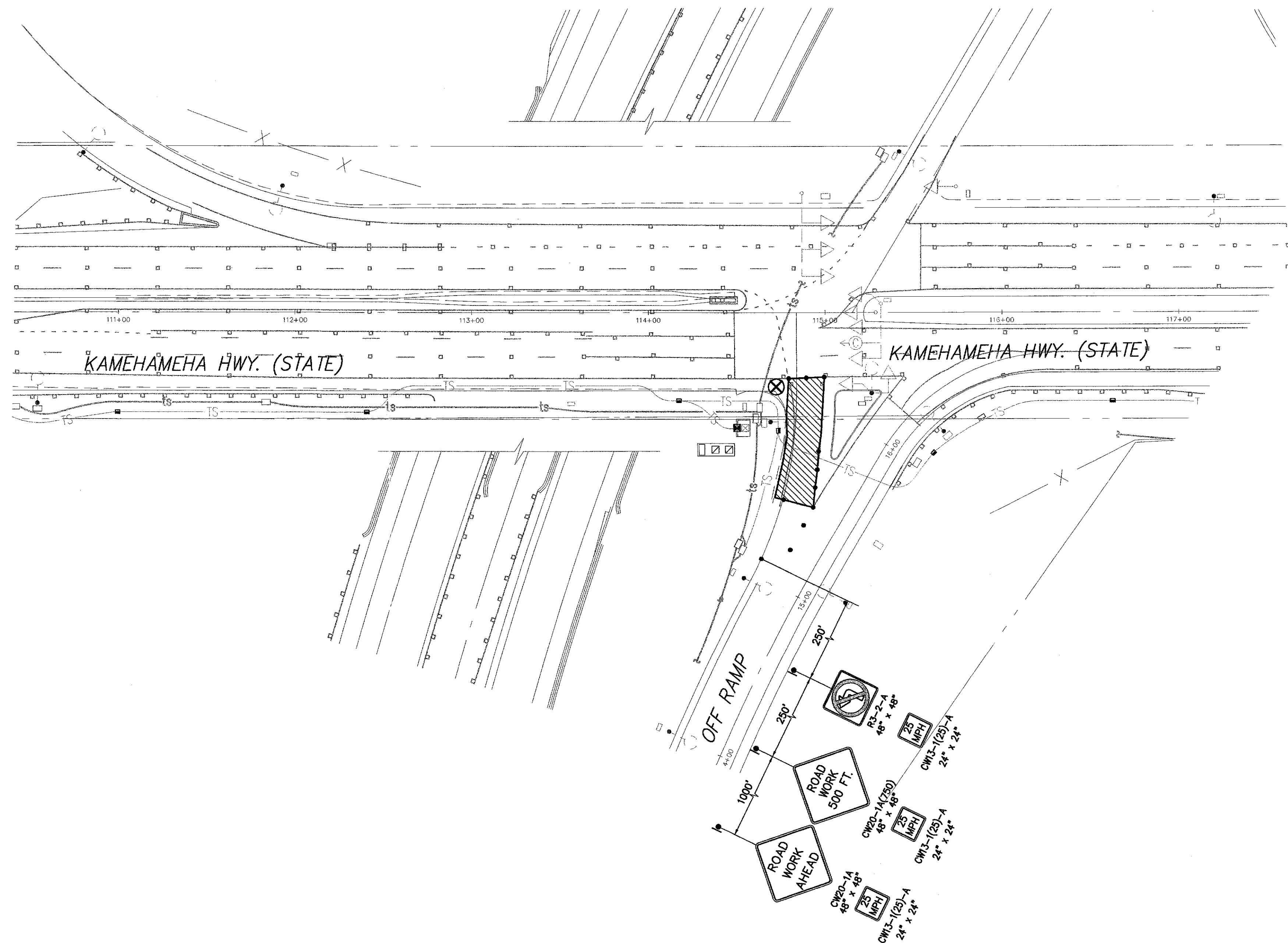
TRAFFIC CONTROL PLAN (HALEKOU INTERCHANGE)-2
