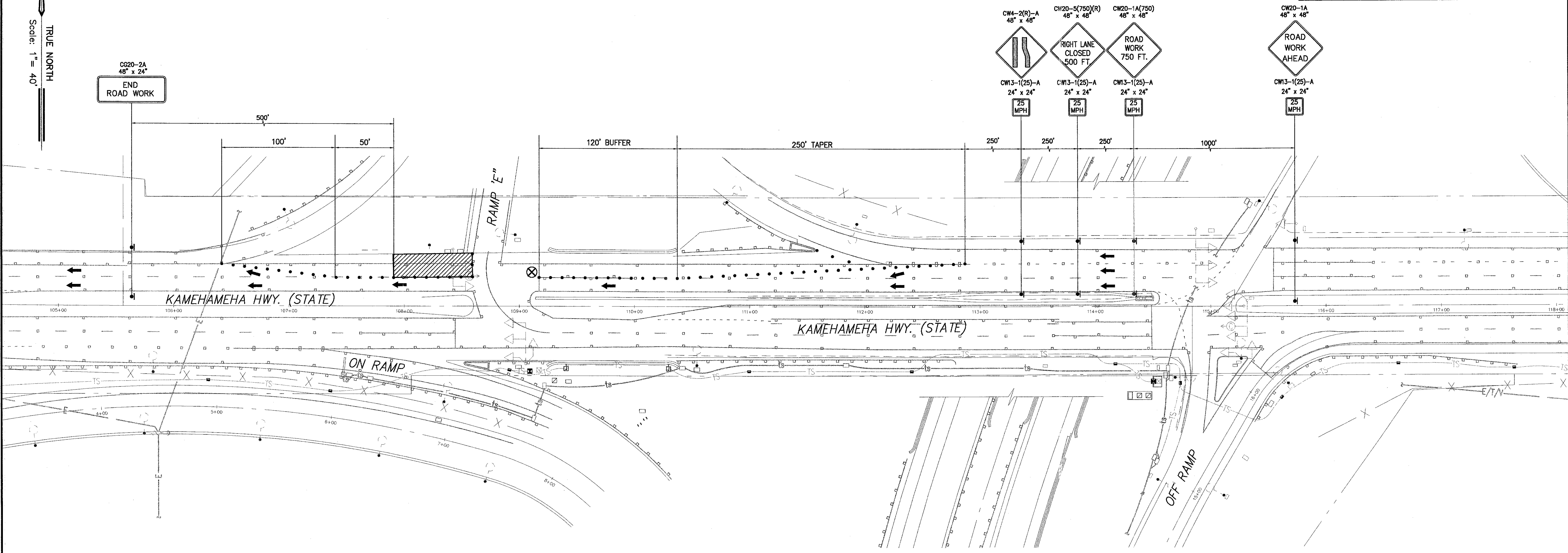
TRAFFIC CONTROL PLAN (HALEKOU INTERCHANGE)-4
