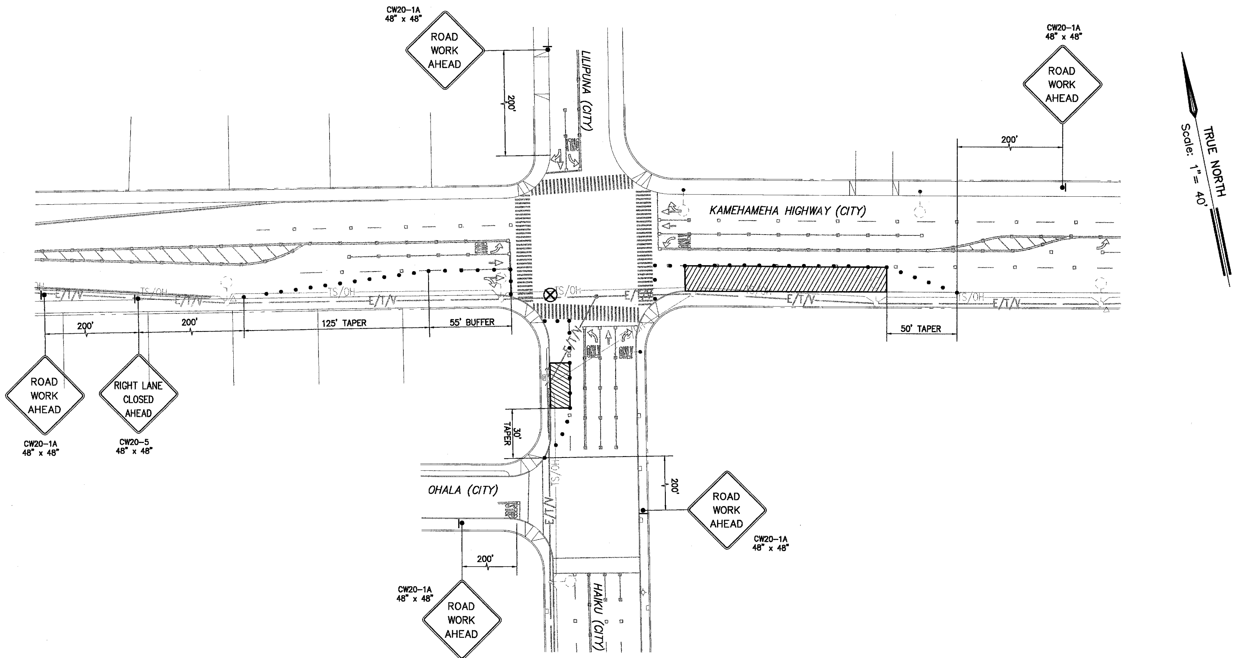
TRAFFIC CONTROL PLAN (HAIKU - KAMEHAMEHA HWY. INTERSECTION)
