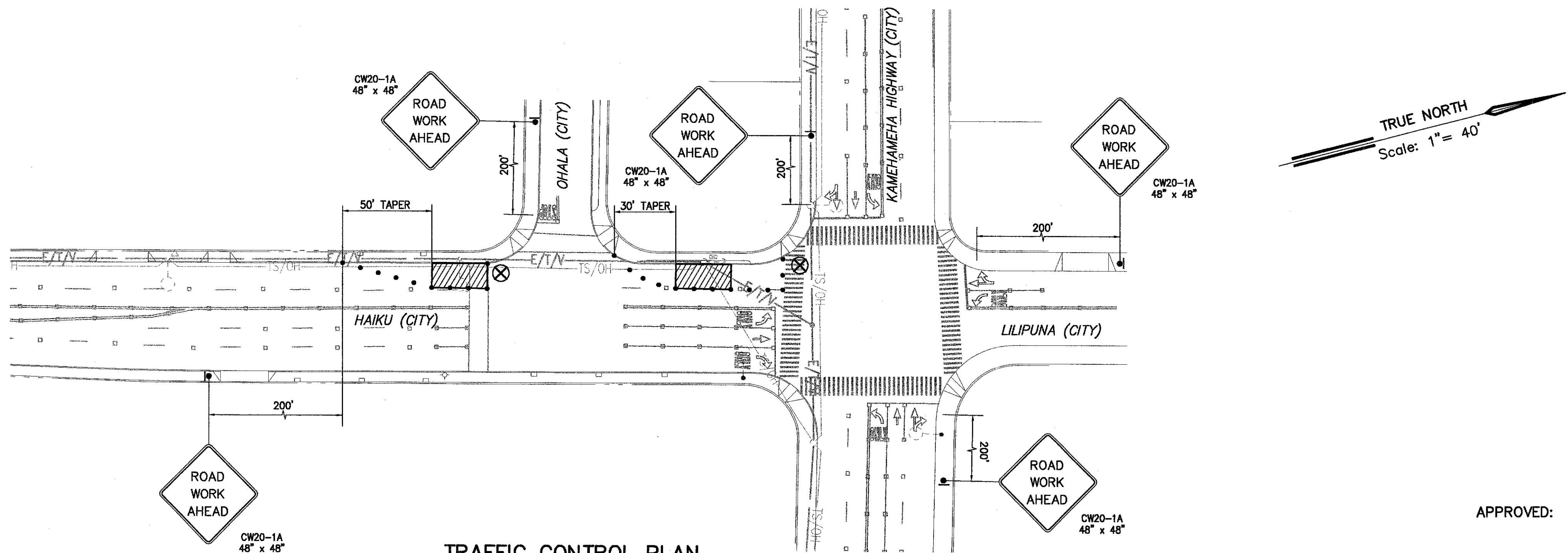
TRAFFIC CONTROL PLAN (HAIKU - OHALA INTERSECTION)-1
