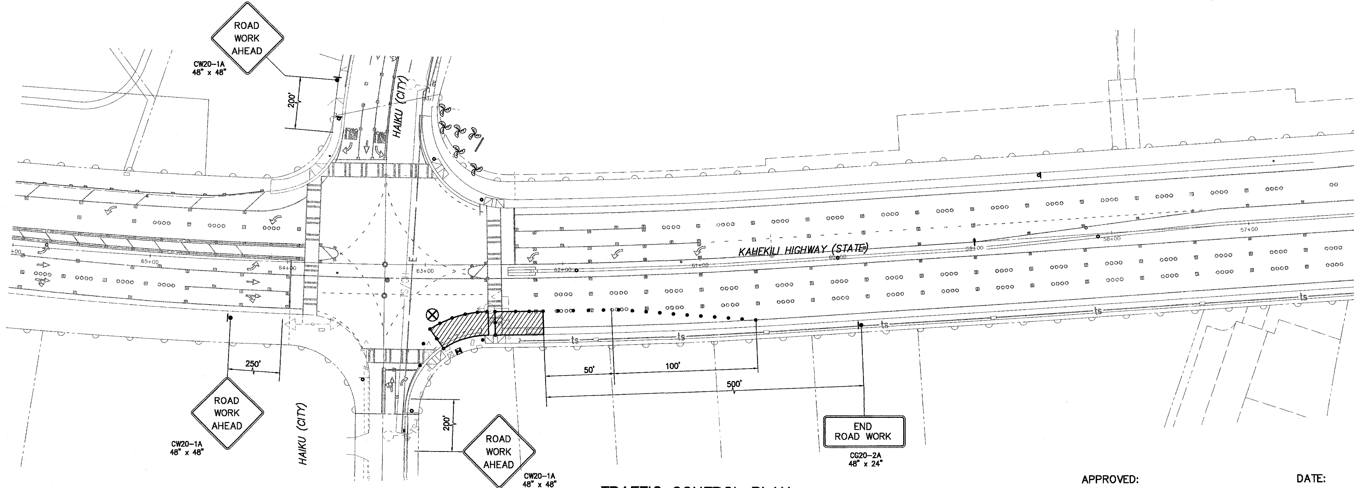
TRAFFIC CONTROL PLAN (HAIKU-KAHEKILI INTERSECTION)-2
