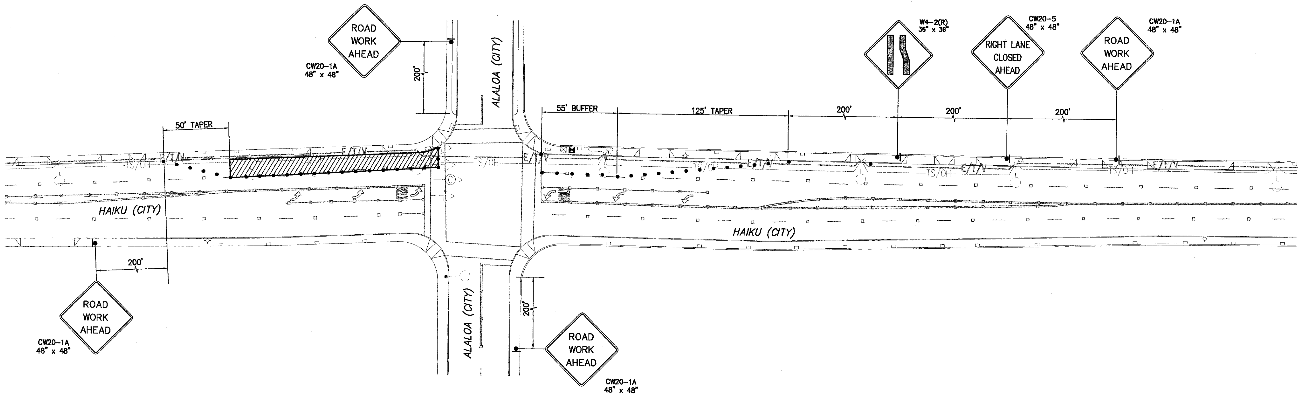
TRAFFIC CONTROL PLAN (HAIKU - ALALOA INTERSECTION)-2
