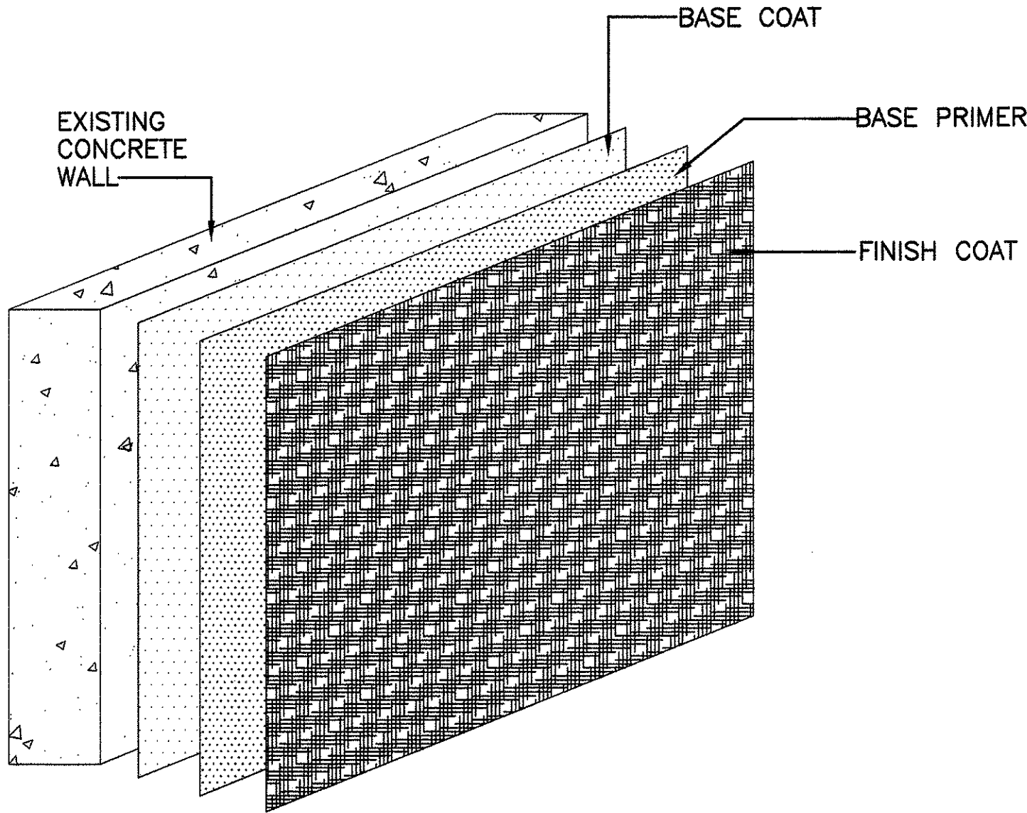
EXTERIOR FINISH SYSTEM (EFS) APPLICATION DETAIL NOT TO SCALE
