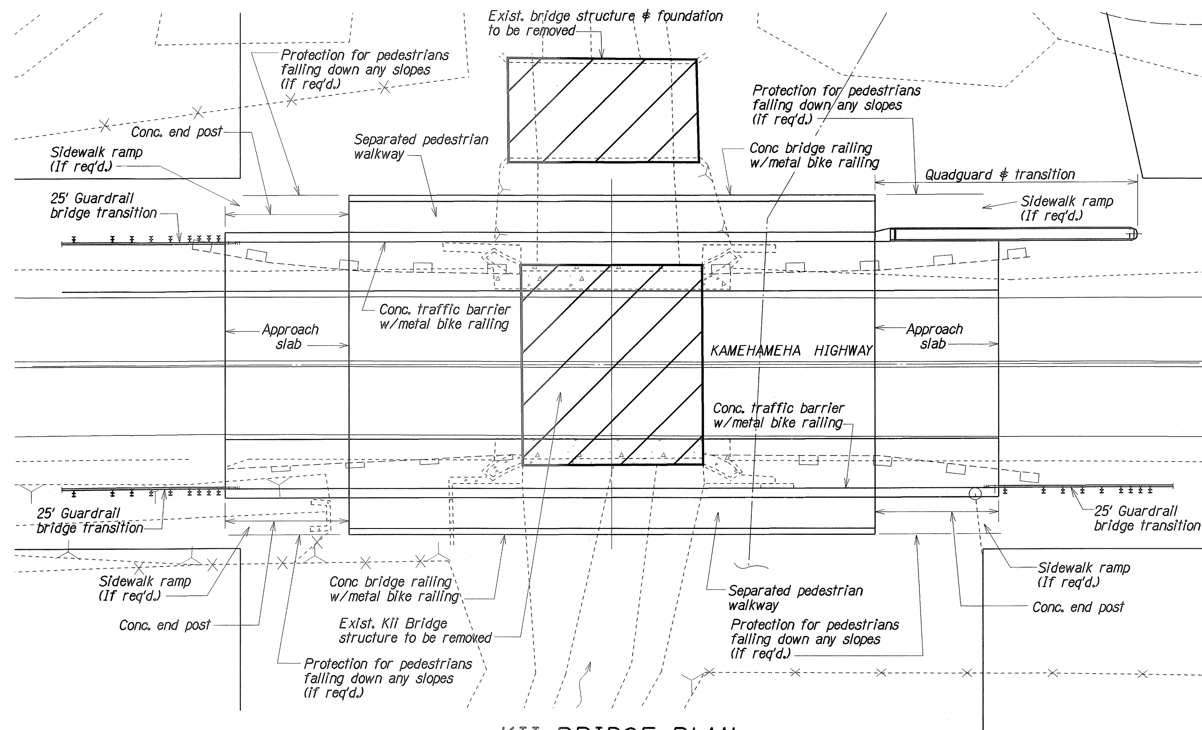
KII BRIDGE PLAN Scale: 1" = 10'-0"
