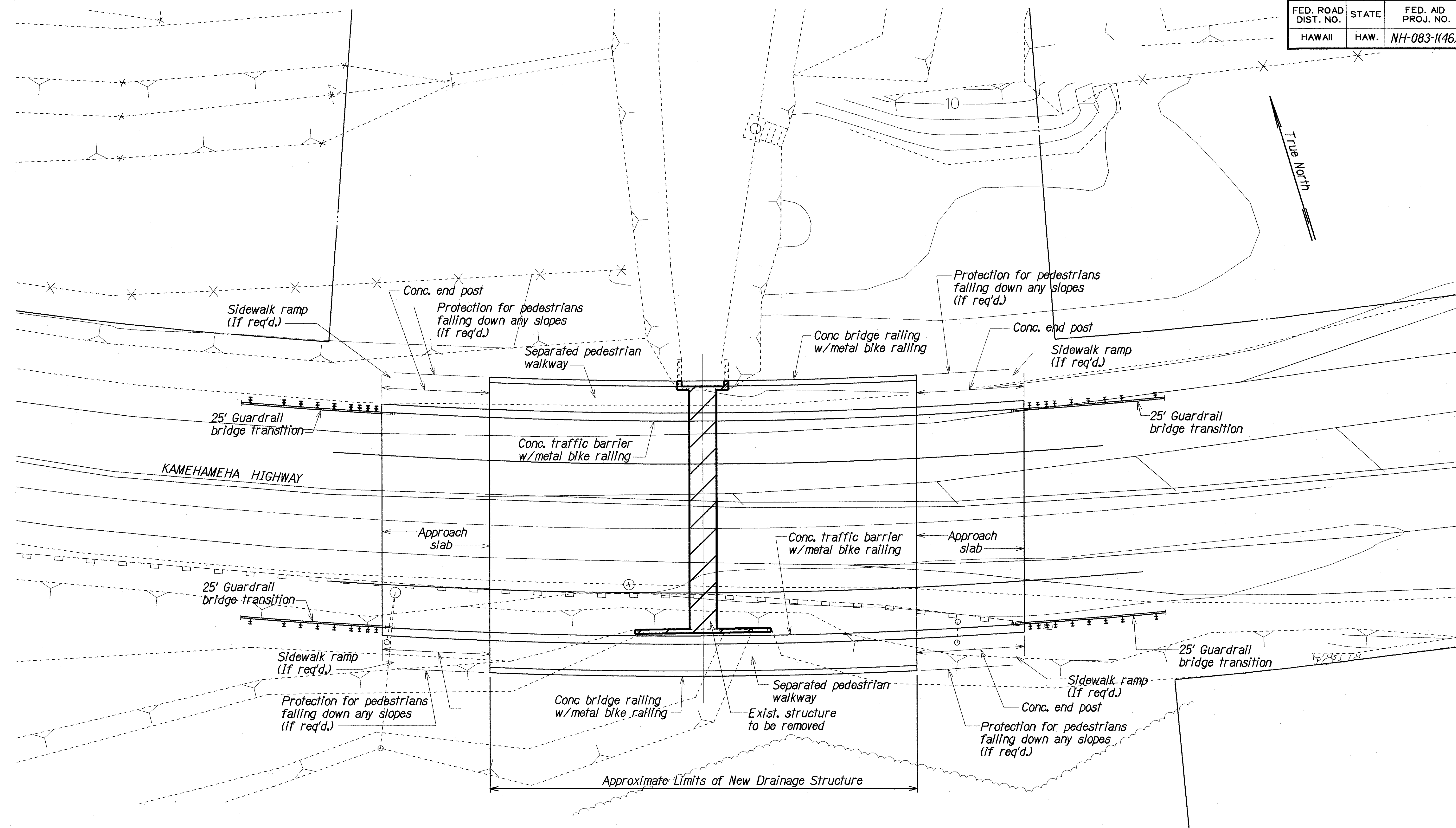
KAHUKU HOSPITAL CULVERT PLAN Scale: 1" = 10'-0"
