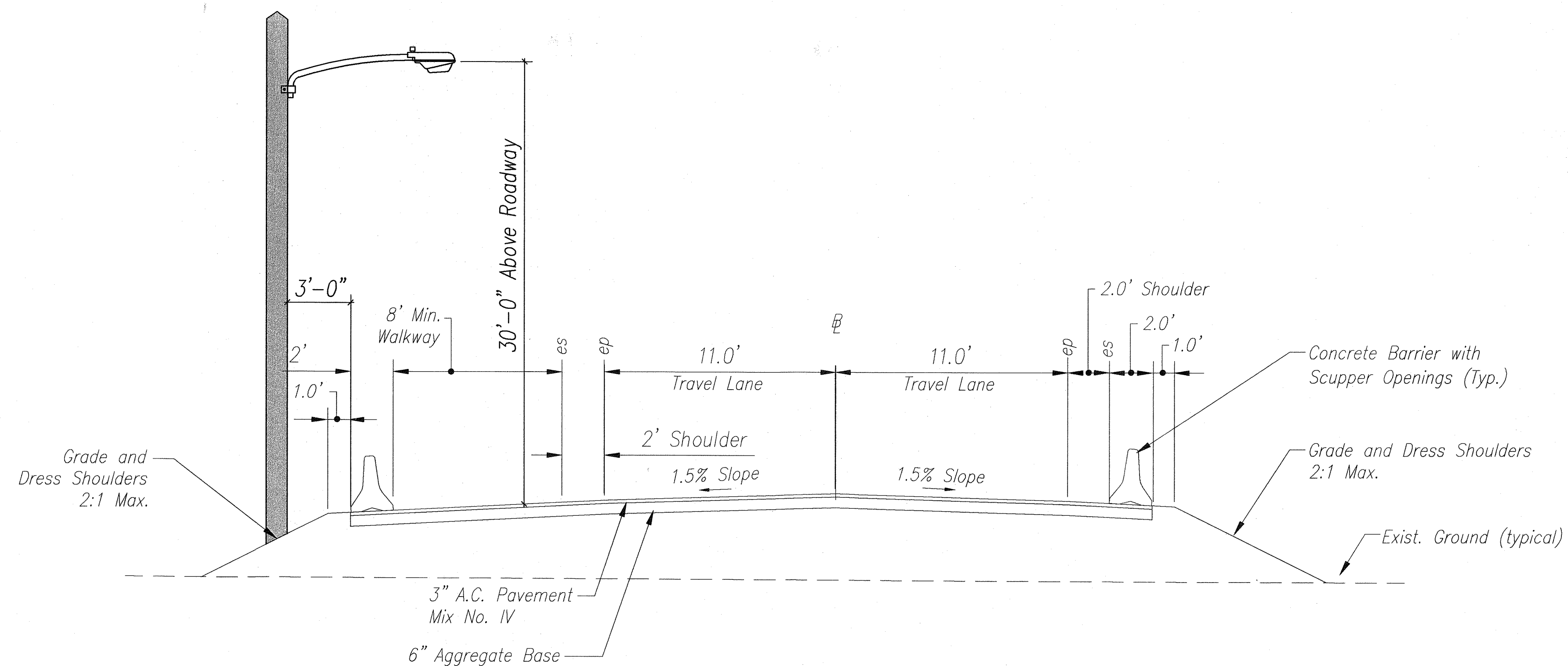
DETOUR ROAD SECTION STREET LIGHT TYPICAL LOCATION NOT TO SCALE
