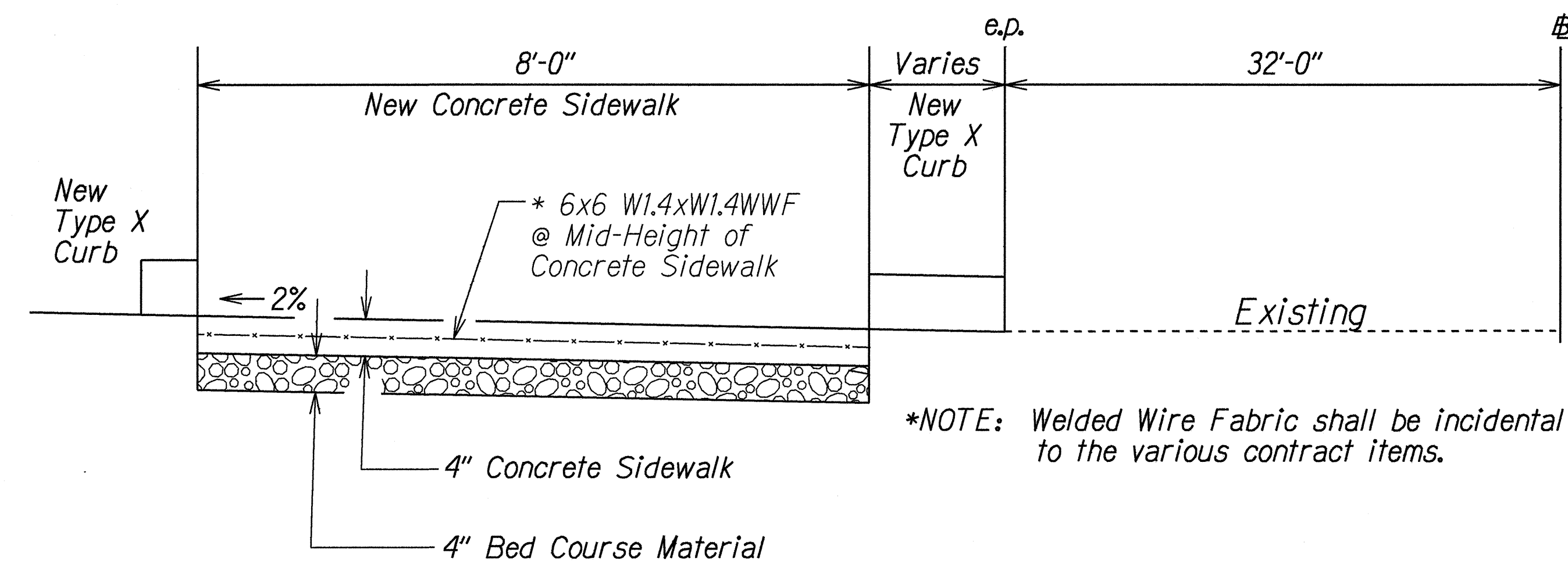
Section B-B
