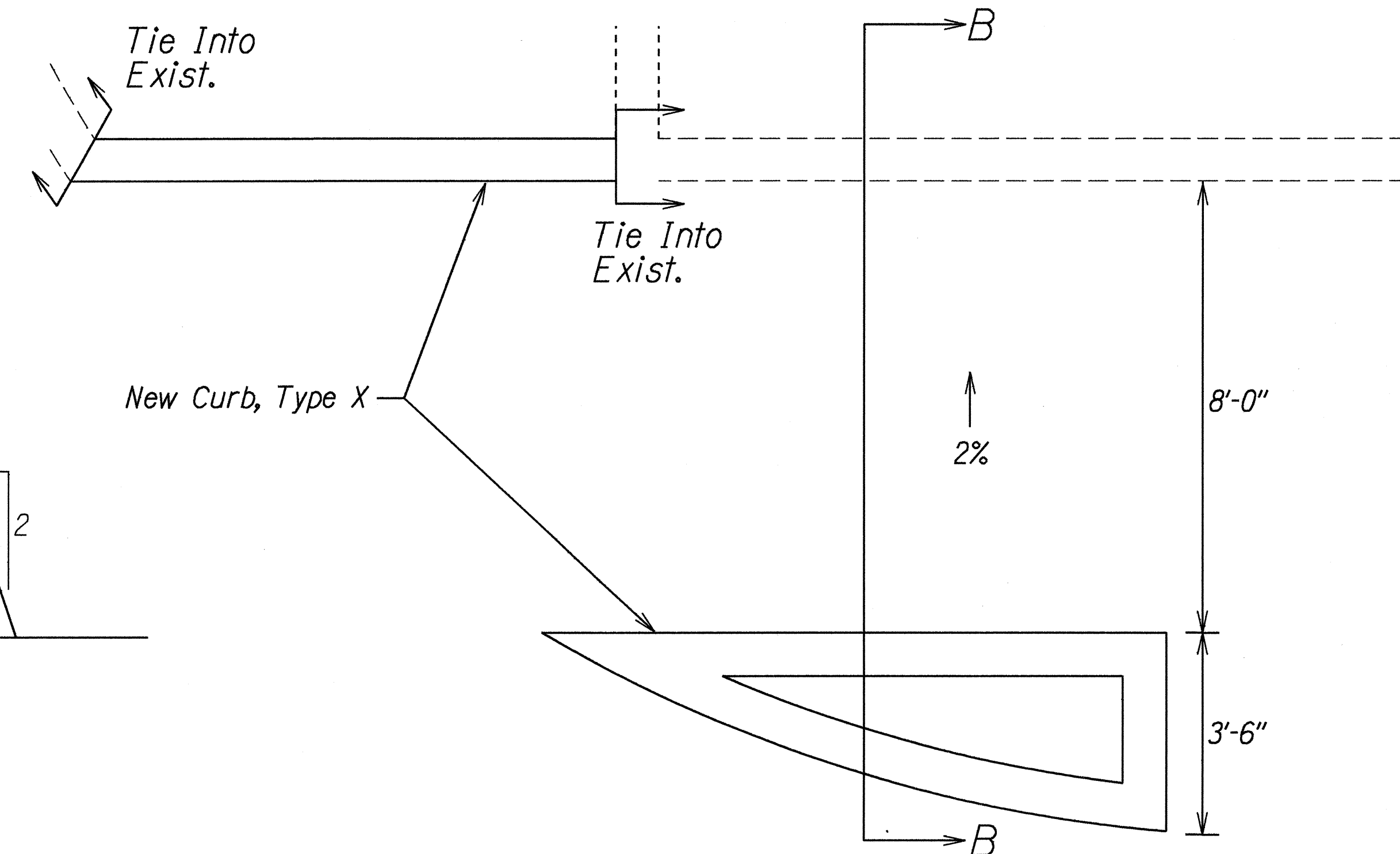
DETAIL @ STA. 1373+50 TO @ STA. 1373+75 Lt.
