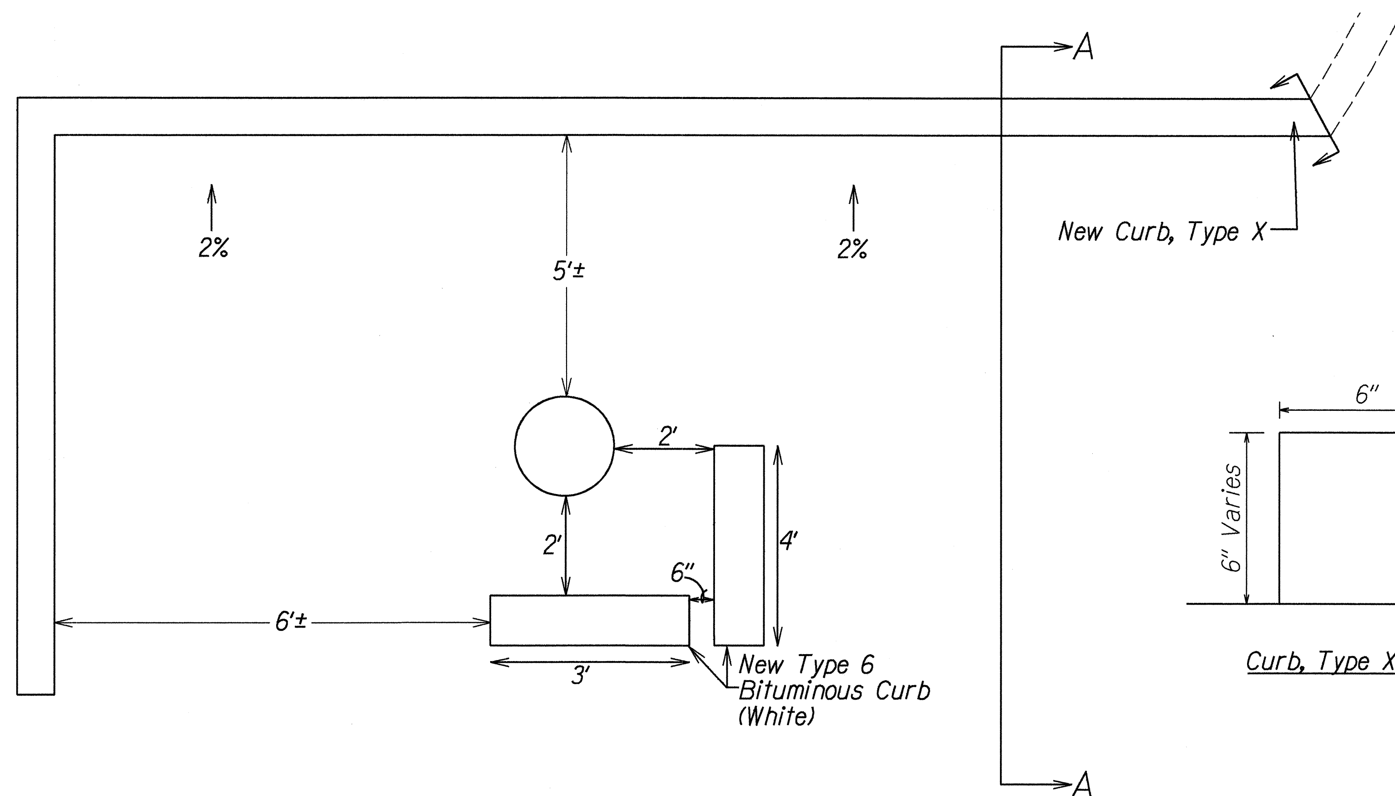
DETAIL @ STA. 1372+86 TO @ STA. 1373+11 Lt.
