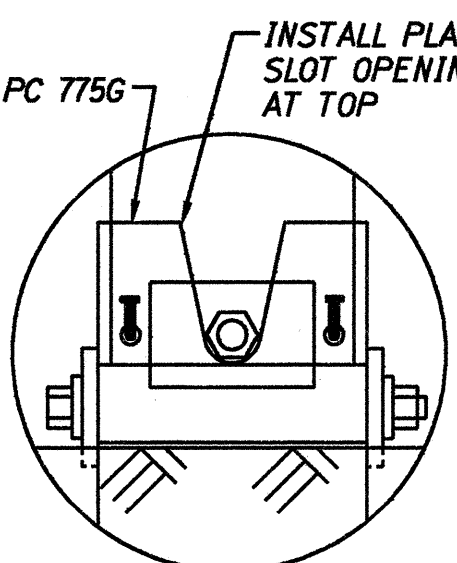
BEARING PLATE ORIENTATION
