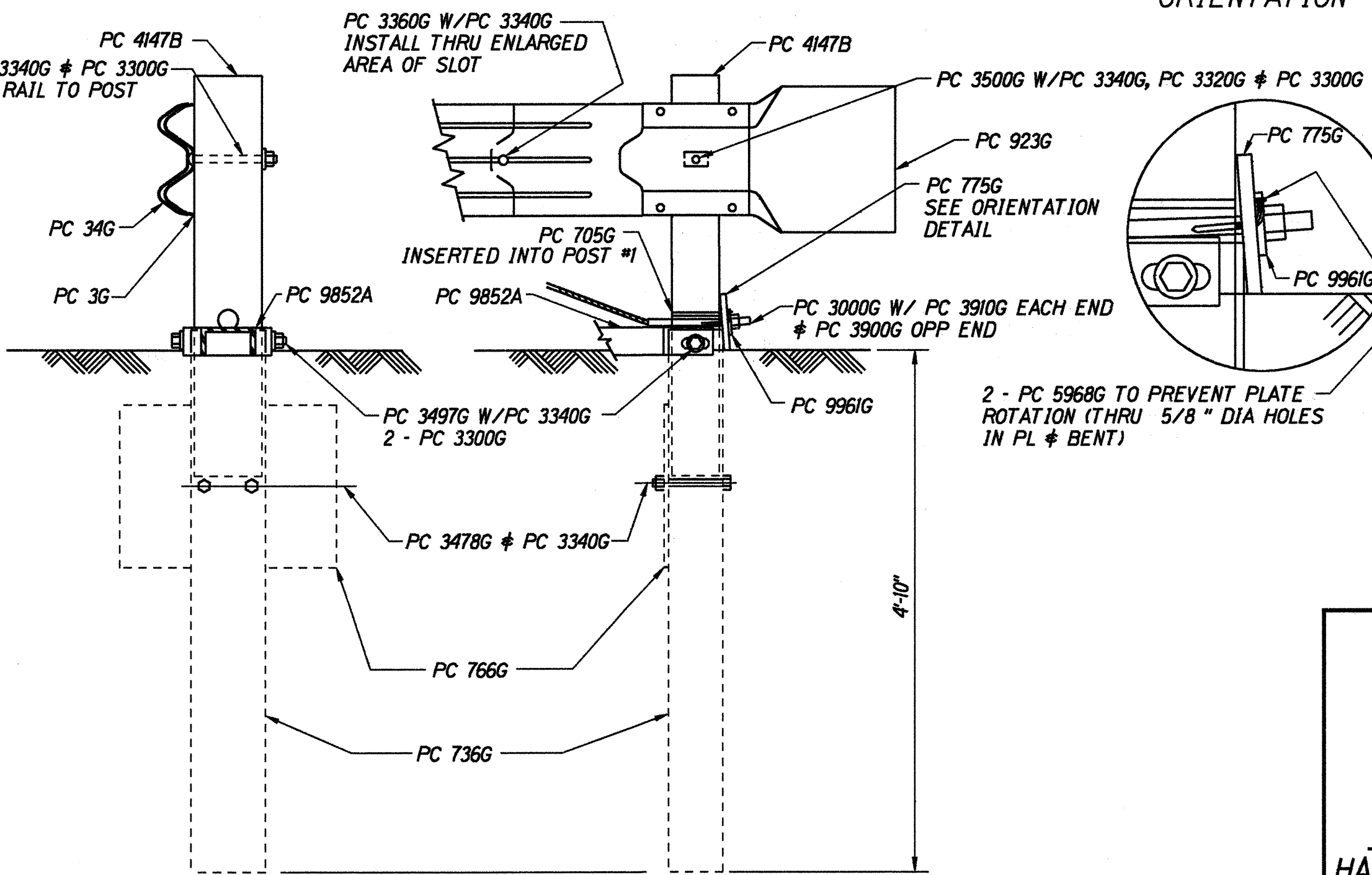
SECTION "A-A" (@ POST #2)
